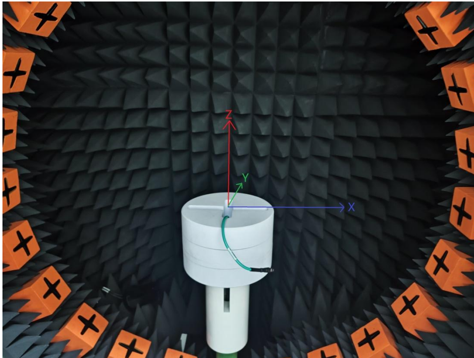
Darkroom direction diagram
