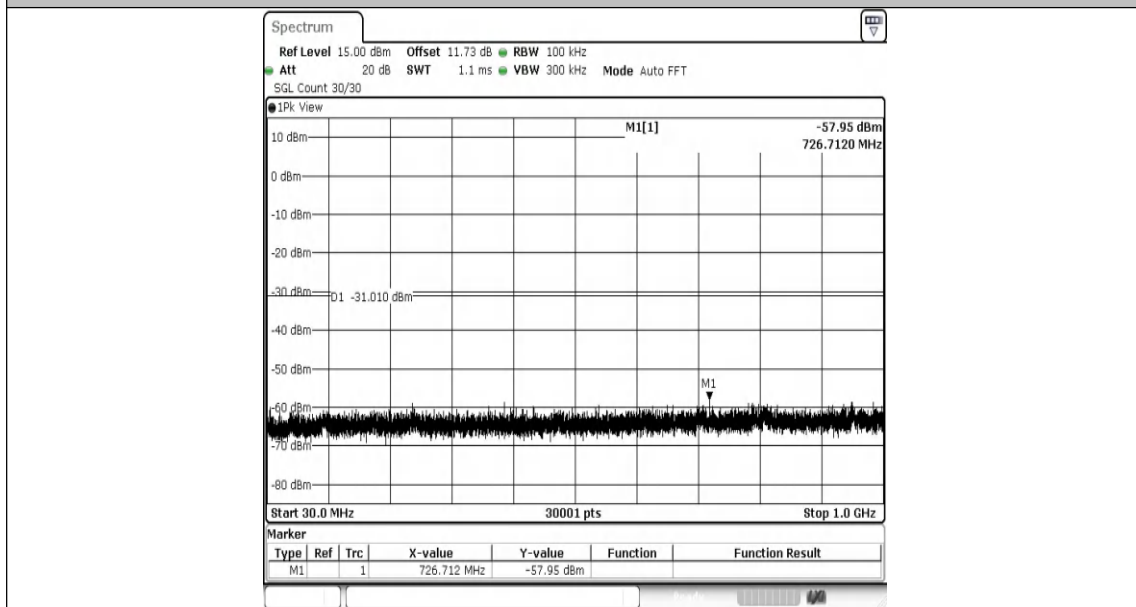
11AX20SISO-Ant1-2462-0~Reference-PASS
