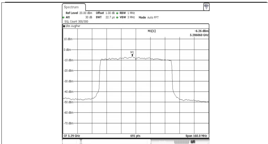
11AX80ISO-Ant1-5290-PASS
