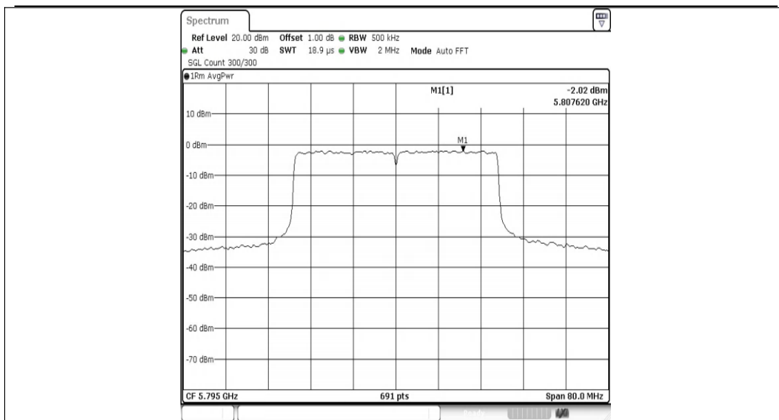
11AX40SISO-Ant1-5795-PASS
