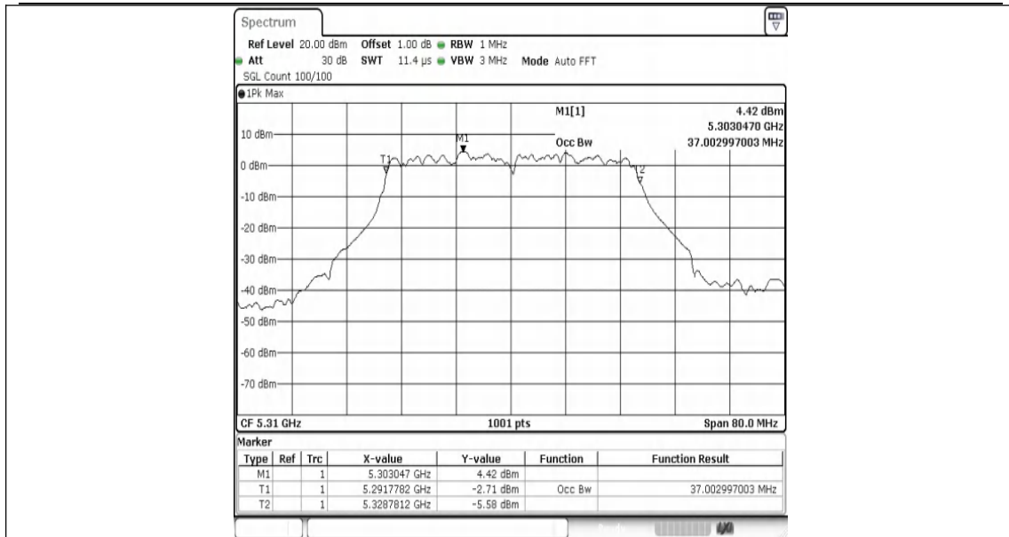
11AC40SISO-Ant1-5310
