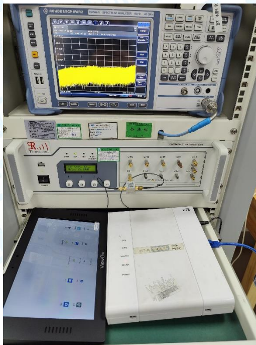
Photo of Setup for DFS Test
