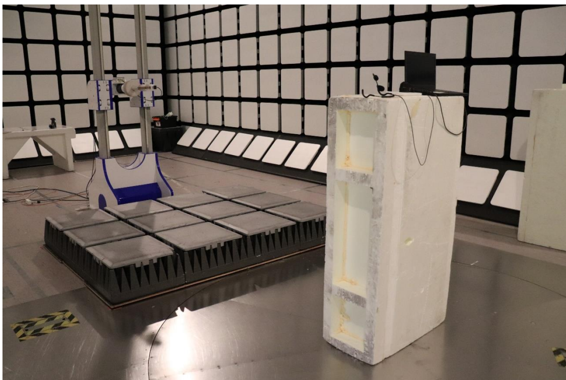
Photograph 6. Test setup for radiated emissions (18 – 25 GHz)
