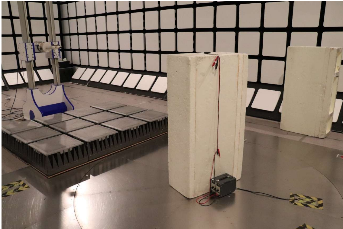
Photograph 5. Test setup for radiated emissions (18 – 26.5 GHz)
