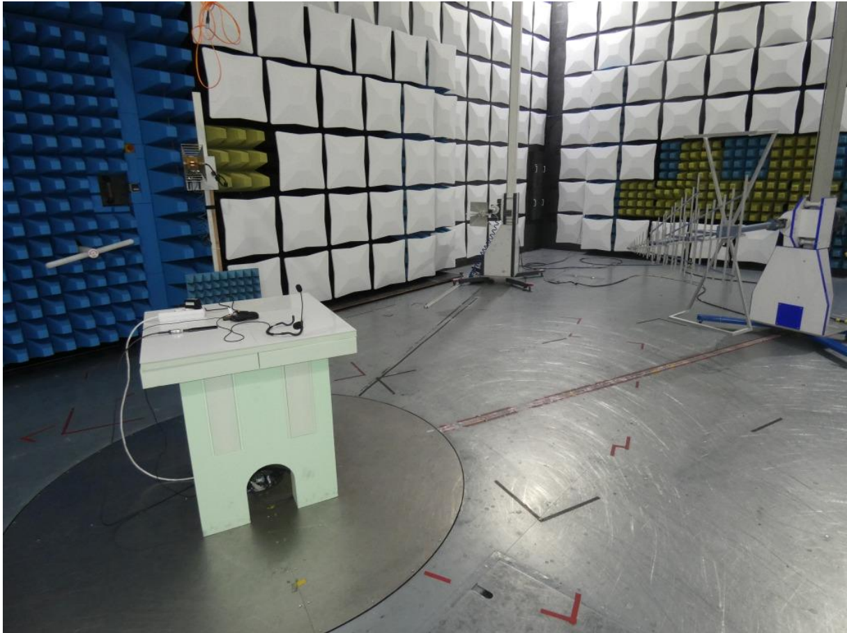
Photo 3: Test setup for radiated measurements (stand alone with AC/DC adapter , semi-anechoic chamber 30 MHz – 1 GHz; unintentional radiator §15.109, ANSI C63.4)
