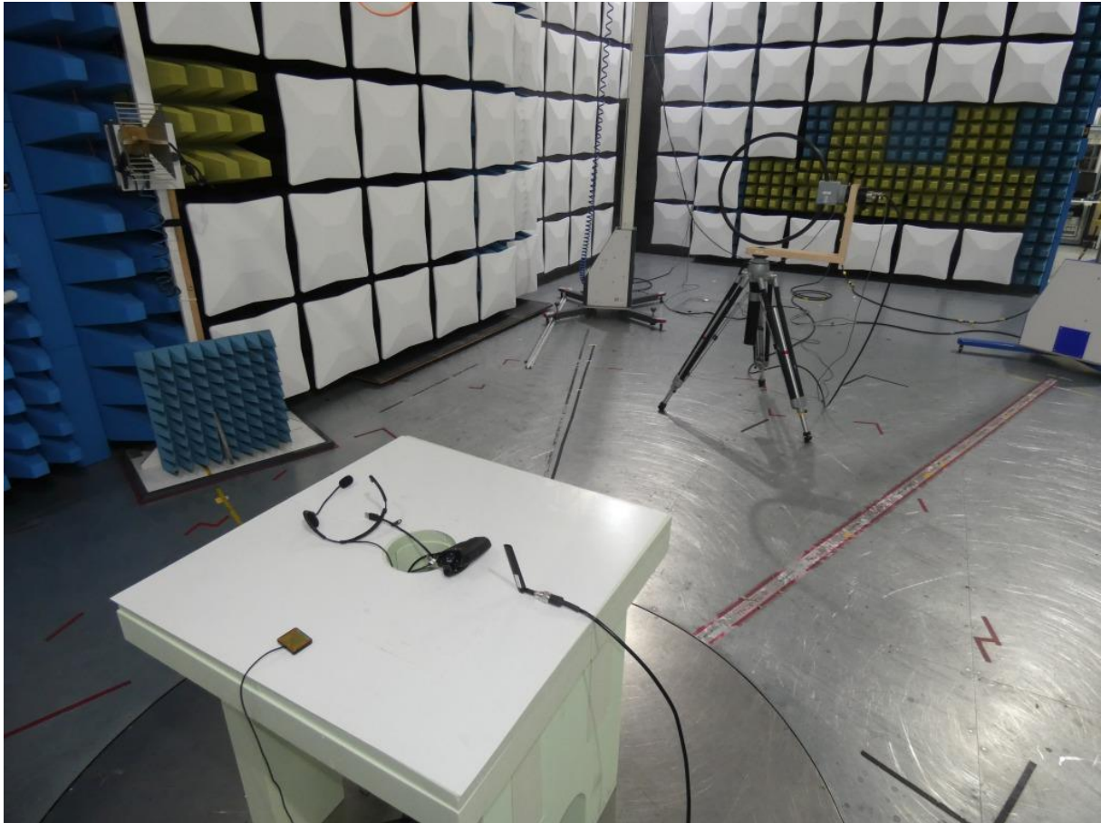
Photo 5: Test setup for radiated measurements (stand alone setup, 9 kHz - 30 MHz; FCC 15c247)
