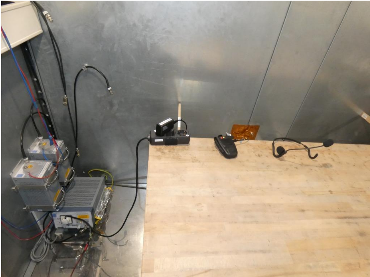
Photo 1: Test setup for conducted measurements (Test Setup: stand alone, AC mains connection: connected via AC/DC adapter, unintentional radiator §15.107, ANSI C63.4)
