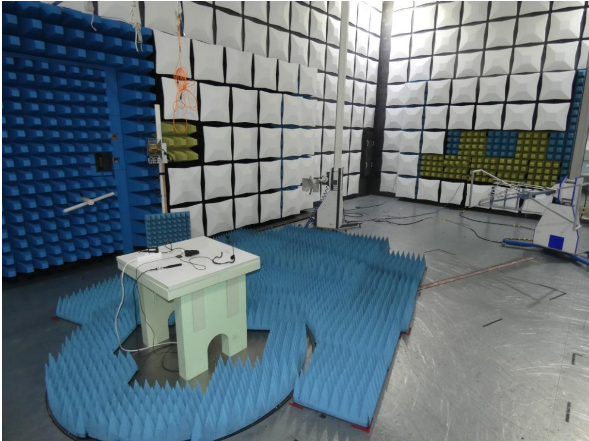
Photo 4: Test setup for radiated measurements (stand alone setup, semi-anechoic chamber above 1 GHz ; unintentional radiator §15.109, ANSI C63.4)
