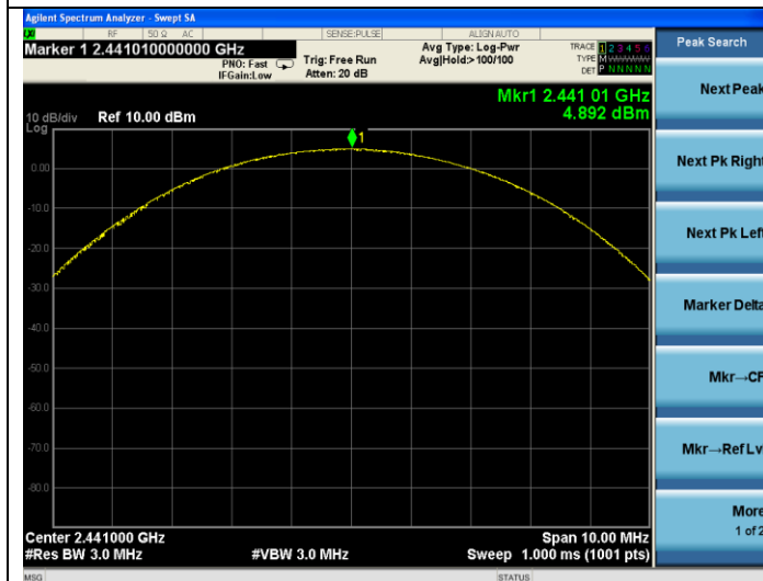
3DH1-Middle channel
