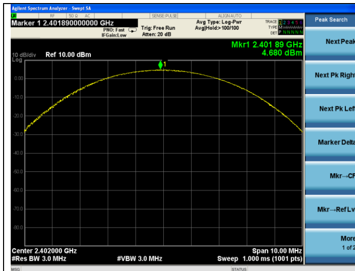
3DH1-Low channel
