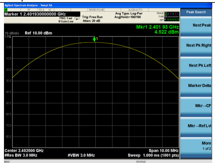
2DH1-Low channel
