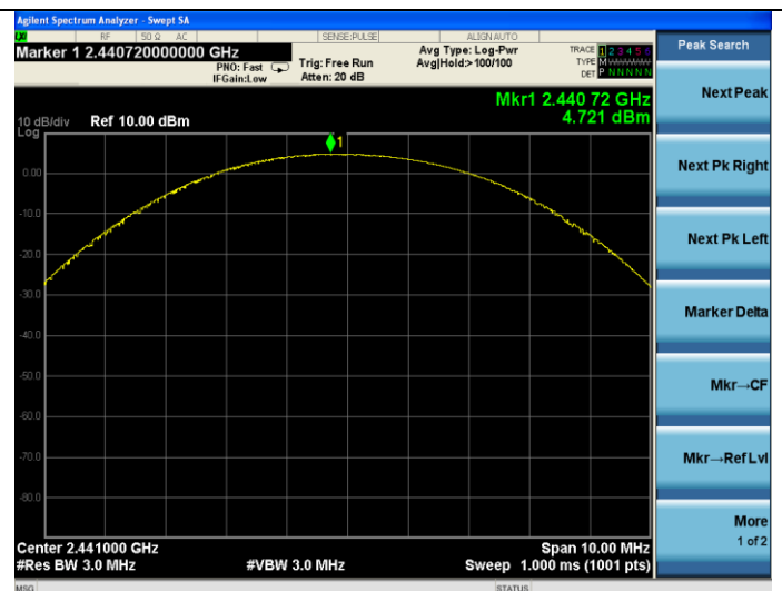
2DH1-Middle channel
