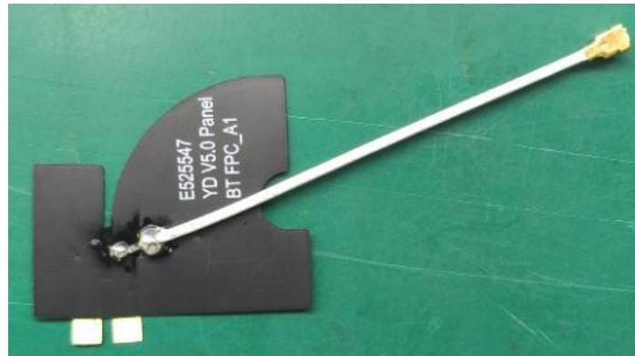
Figure 1 Antenna
