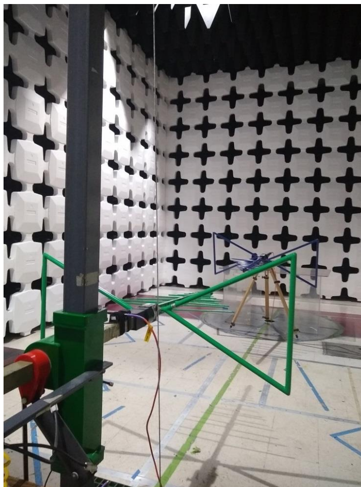
Figure 3: Substitution Method, Below 1GHz, Test Setup
