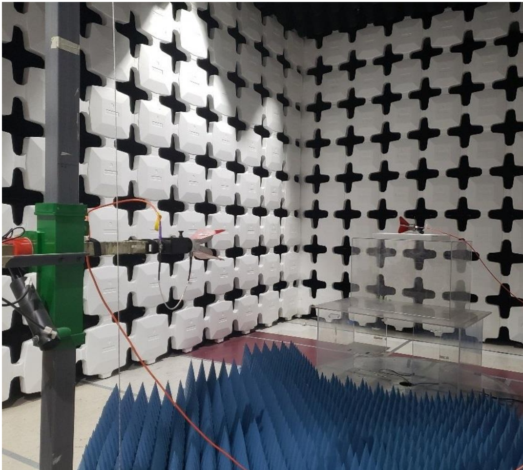
Figure 4: Substitution Method, Above 1GHz, Test Setup
