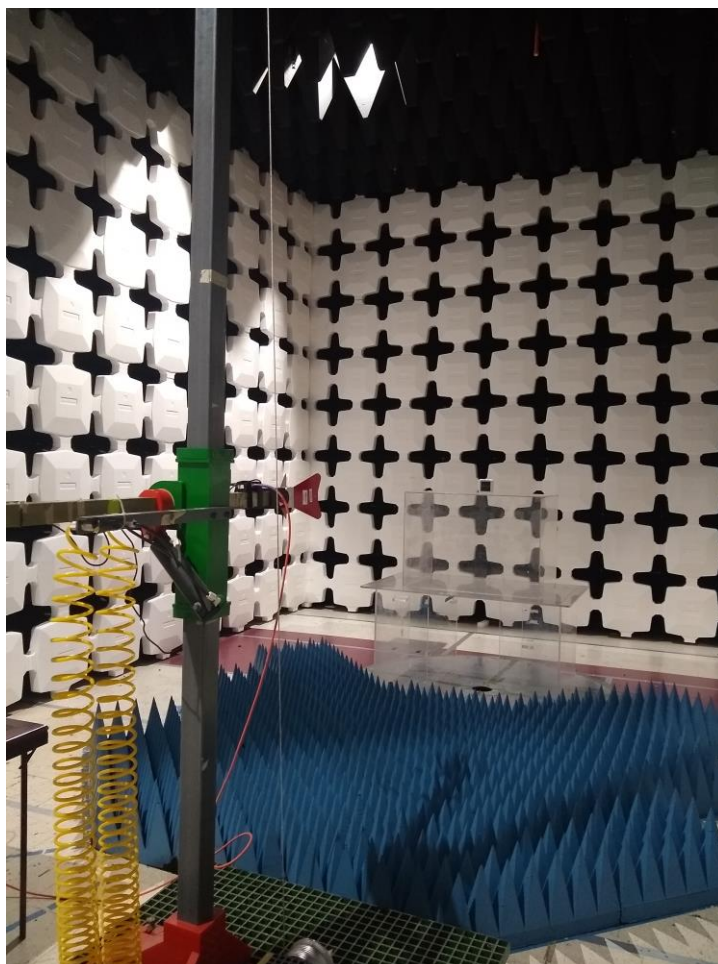
Figure 2: Radiated Spurious Emissions, 1GHz-18GHz, Test Setup
