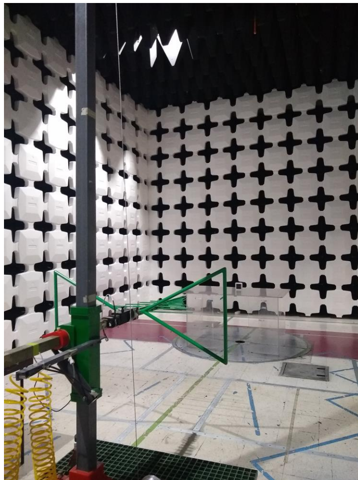
Figure 1: Radiated Spurious Emissions, 30MHz-1GHz, Test Setup
