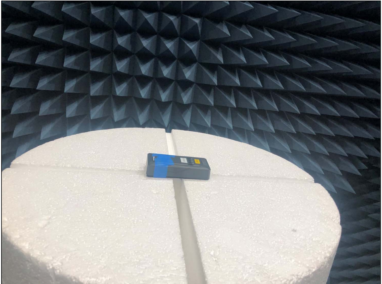
OTA EIRP Measurement, Test Setup, View 2
