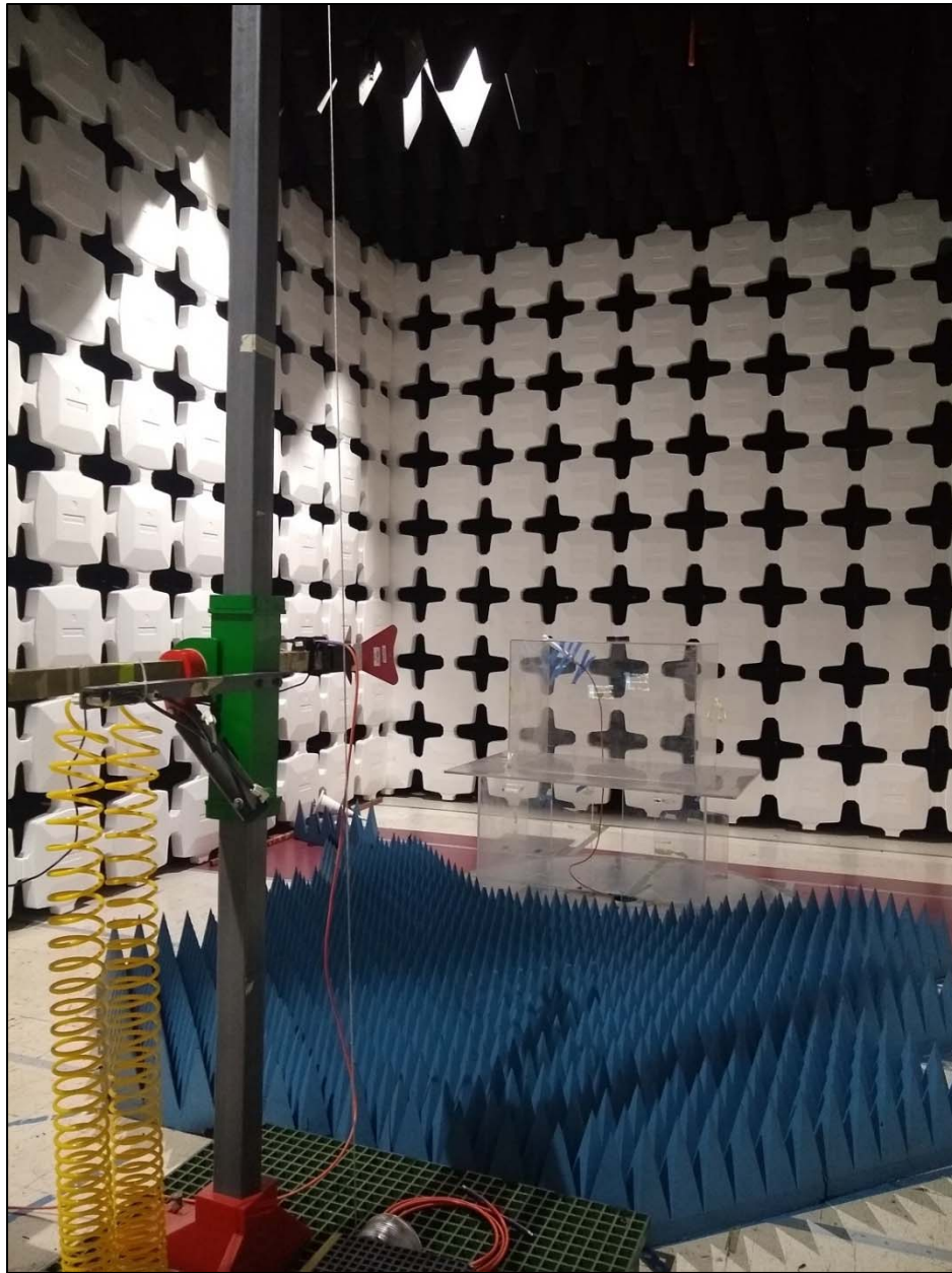
Radiated Spurious Emissions, 1GHz – 18GHz, Test Setup
