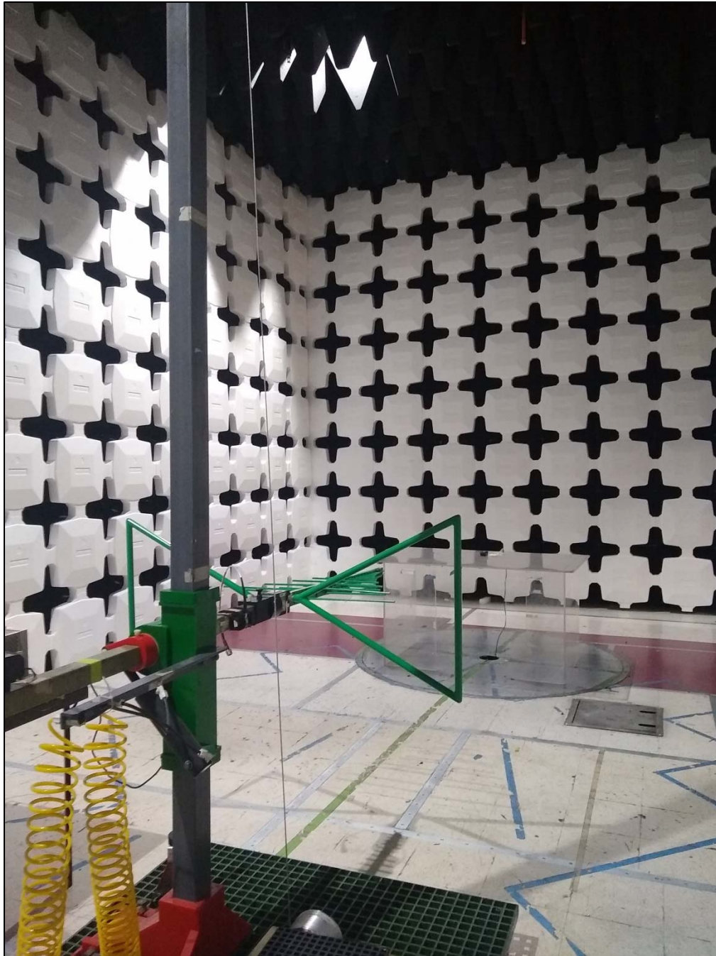
30MHz – 1GHz, Part15B Test Setup
