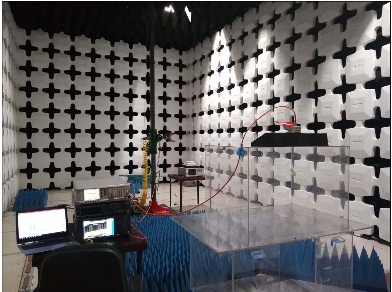
Substitution Method, Test Setup
