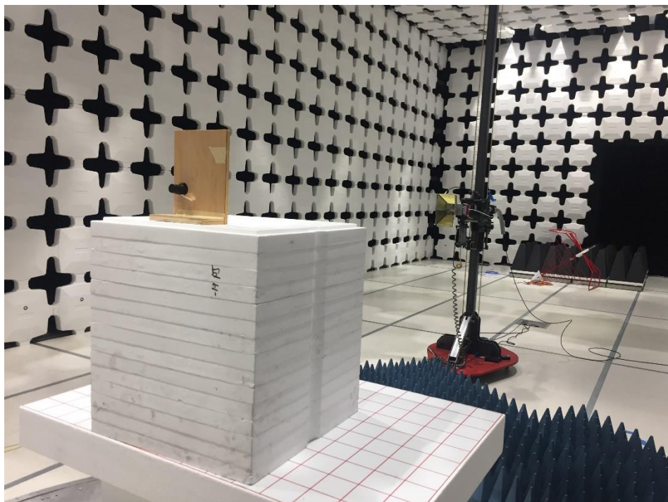
Radiated Emissions Above 1GHz setup for intentional radiator – Rear
