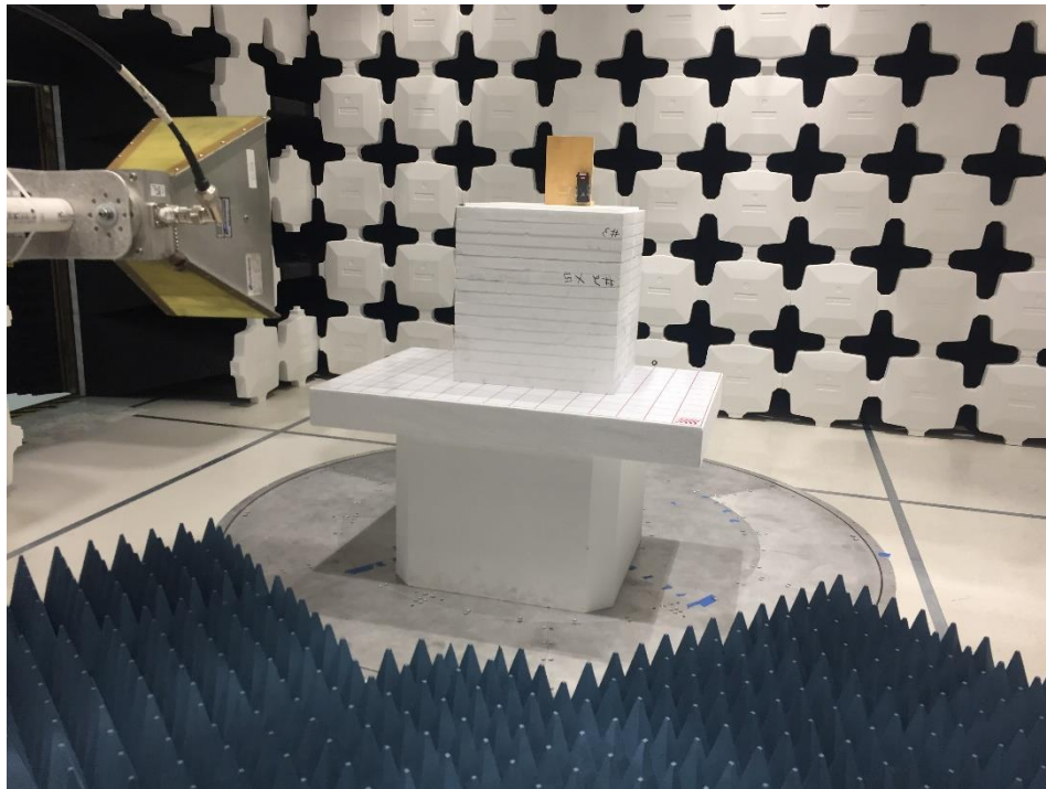
Radiated Emissions Above 1GHz setup for intentional radiator – Front
