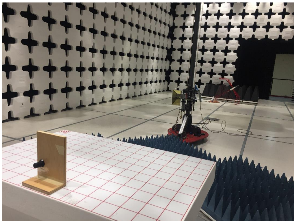
Radiated Emissions Above 1GHz setup for unintentional radiator – Rear
