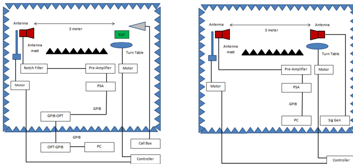
Figure 2. ERP / EIRP, Block Diagram, Test Setup Above 1GHz
