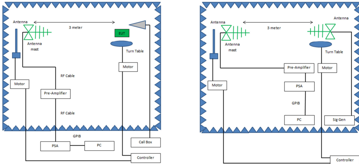
Figure 1. ERP / EIRP, Block Diagram, Test Setup Below 1GHz
