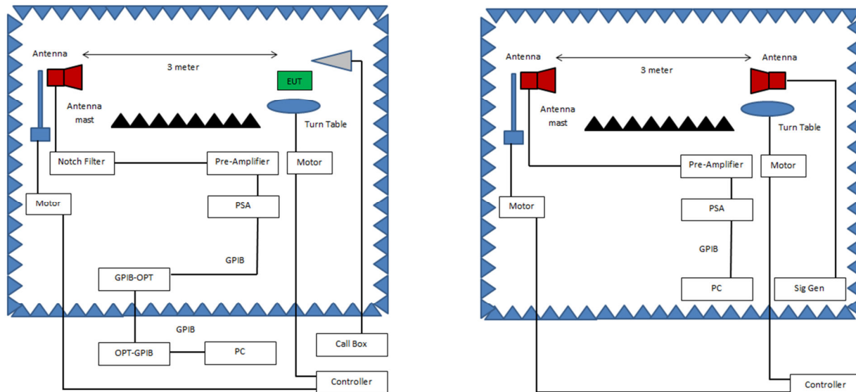
Figure 2. ERP / EIRP, Block Diagram, Test Setup Above 1GHz
