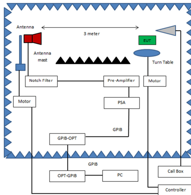
Figure 3. Radiated Spurious Emissions, Block Diagram, Test Setup
