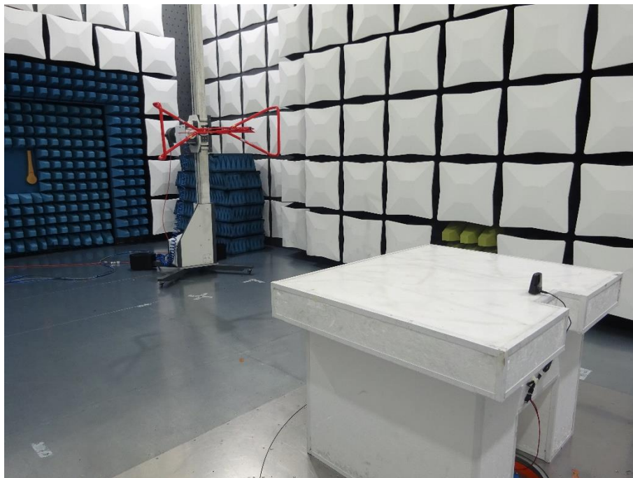
SET UP FOR RADIATED EMISSION TEST (below 1GHz)
