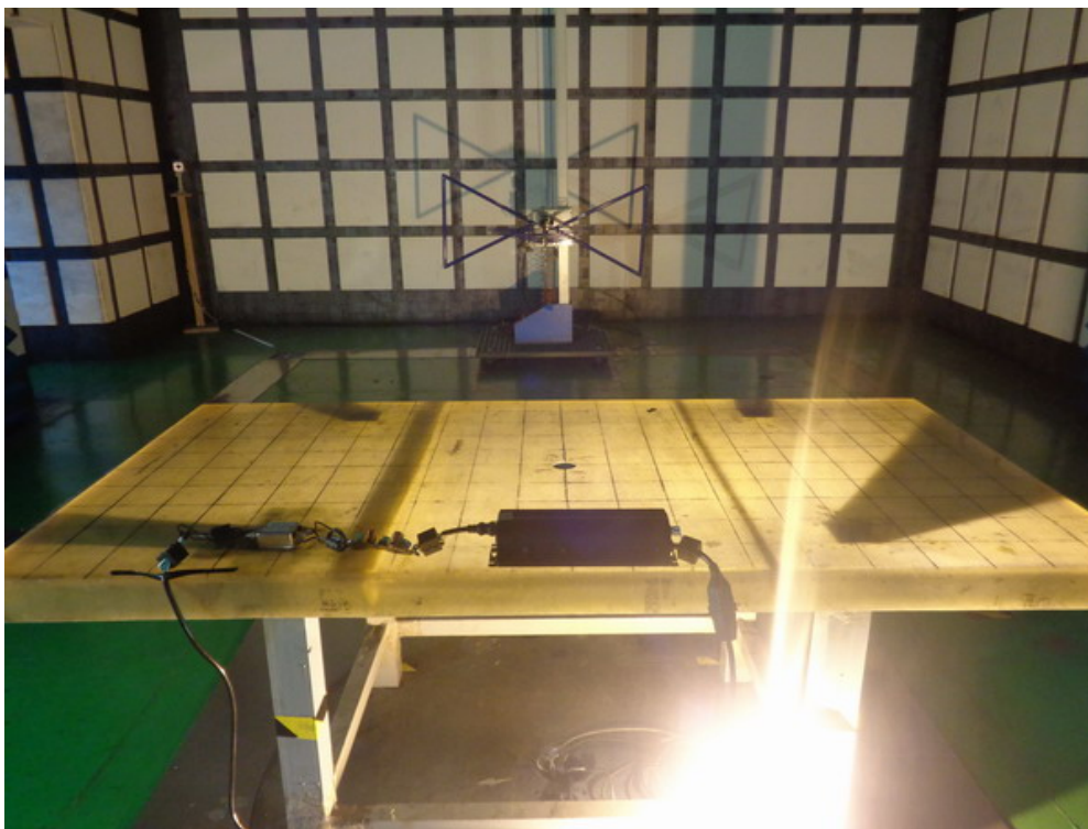
Photograph 3: Radiated Emission Test Configuration, (30-1000MHz), Front
