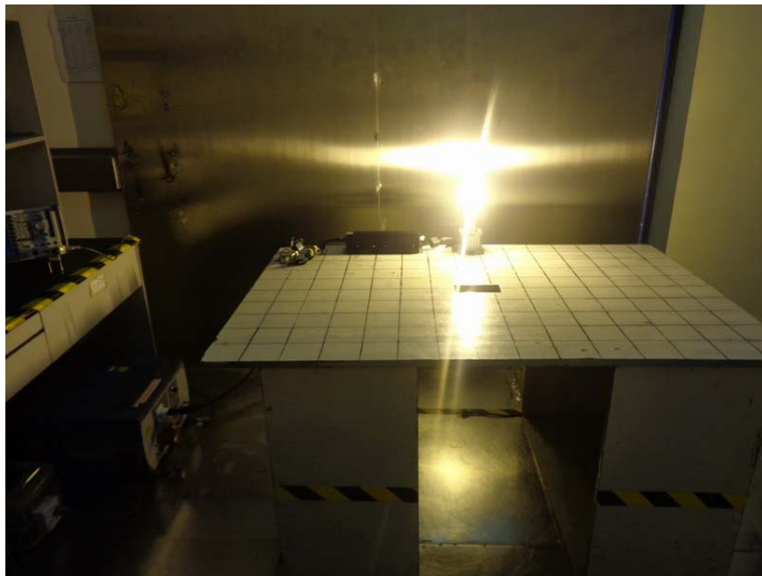
Photograph 1: Conducted Emissions Front
