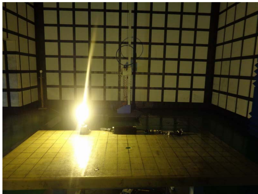
Photograph 4: Radiated Emission Test Configuration, (9kHz-30MHz)
