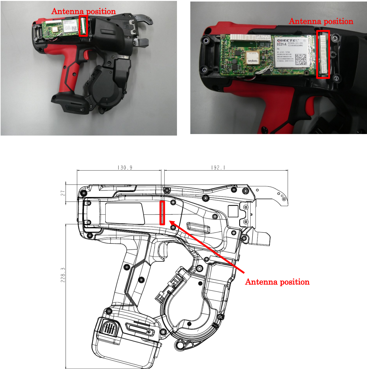
Figure 2 – Picture of the antenna position (DUT)
