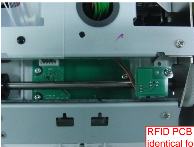
Fig.10. RFID circuit board (CPM-100HG5U) focus
