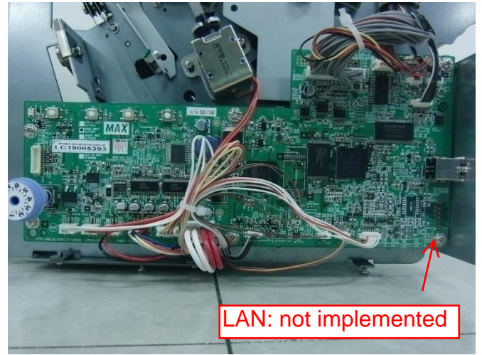
Fig.13. Main circuit board (CPM-100G5U) View
