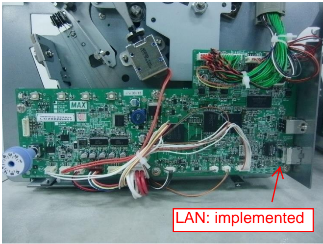
Fig.12. Main circuit board (CPM-100HG5U) View
