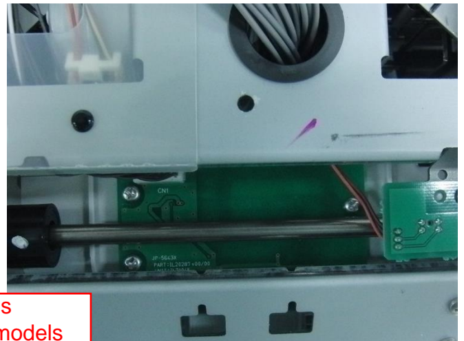
Fig.11. RFID circuit board (CPM-100G5U) focus
