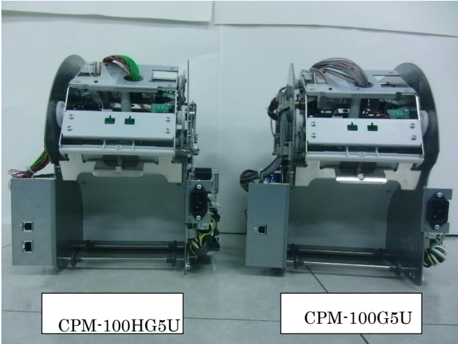
Fig.1. Front view
