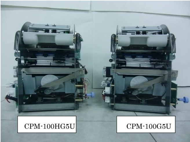
Fig.3. Back view
