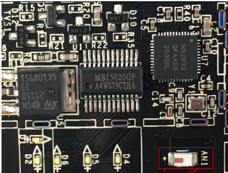
Ceramic Antenna
