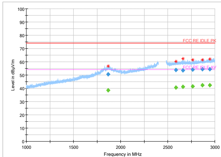
Fig.75 Radiated Spurious Emission (802.11 n-40MHz,Ch9,1GHz~3GHz)
