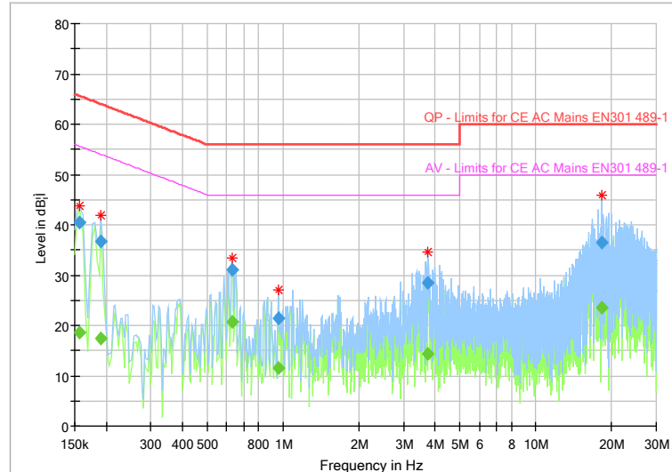
Fig.78 AC Power line Conducted Emission
