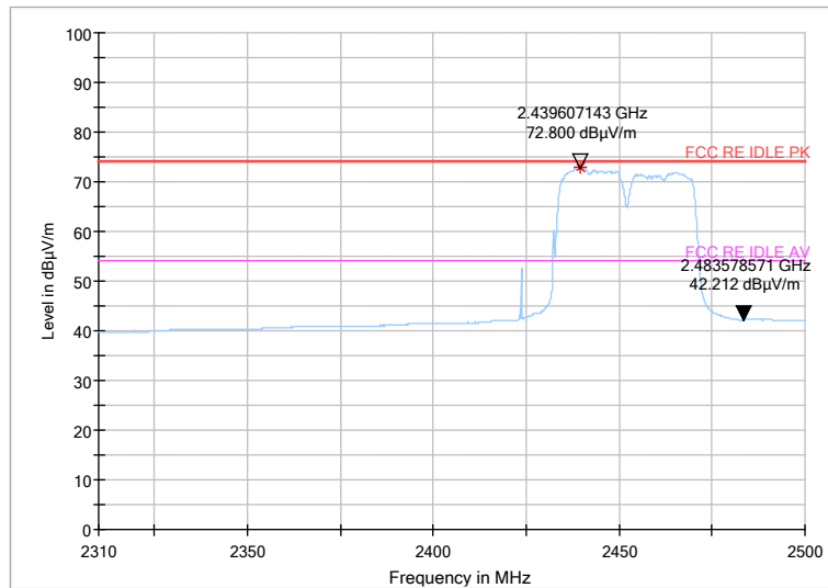
Fig.73 Radiated emission (Power): 802.11n (40M) , high channel
