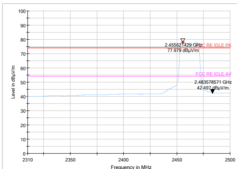
Fig.68 Radiated emission (Power): 802.11n, high channel
