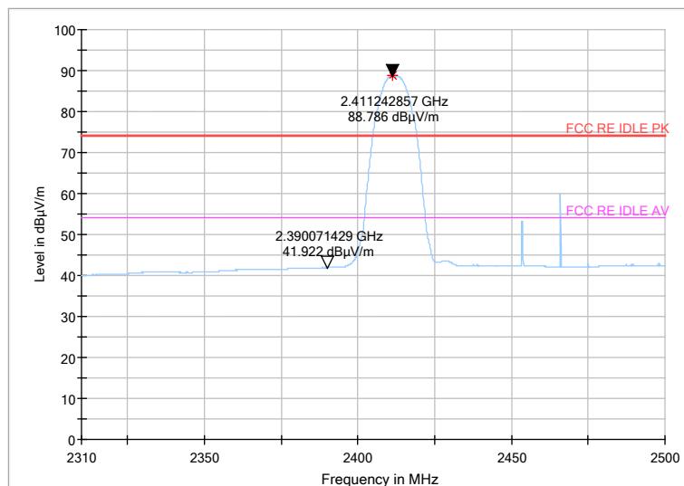
Fig.57 Radiated emission (Power): 802.11b, low channel
