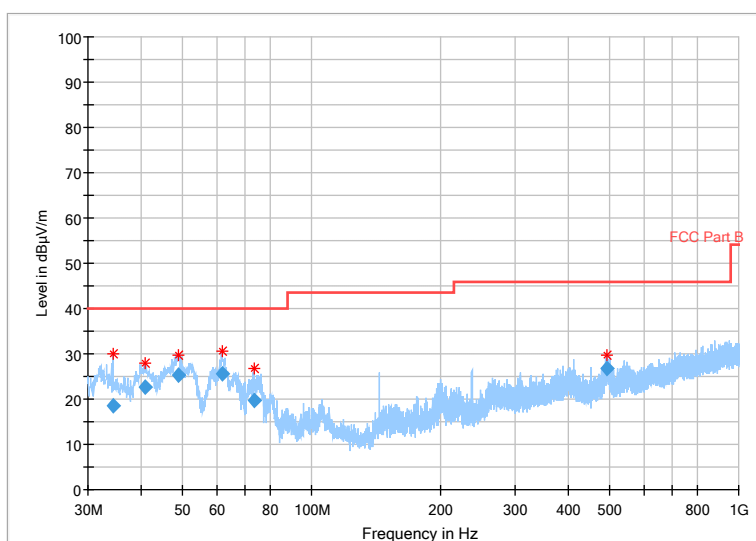
Fig.69 Radiated Spurious Emission (802.11 n-20MHz,Ch1,30MHz~1GHz)
