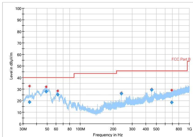
Fig.74 Radiated Spurious Emission (802.11 n-40MHz,Ch9,30MHz~1GHz)
