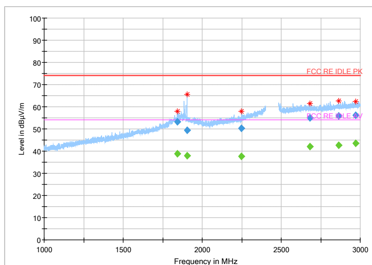
Fig.65 Radiated Spurious Emission (802.11g,Ch11,1GHz~3GHz)
