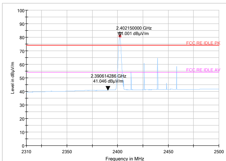
Fig.48 Radiated emission (Power): \pi/4 DQPSK, low channel
