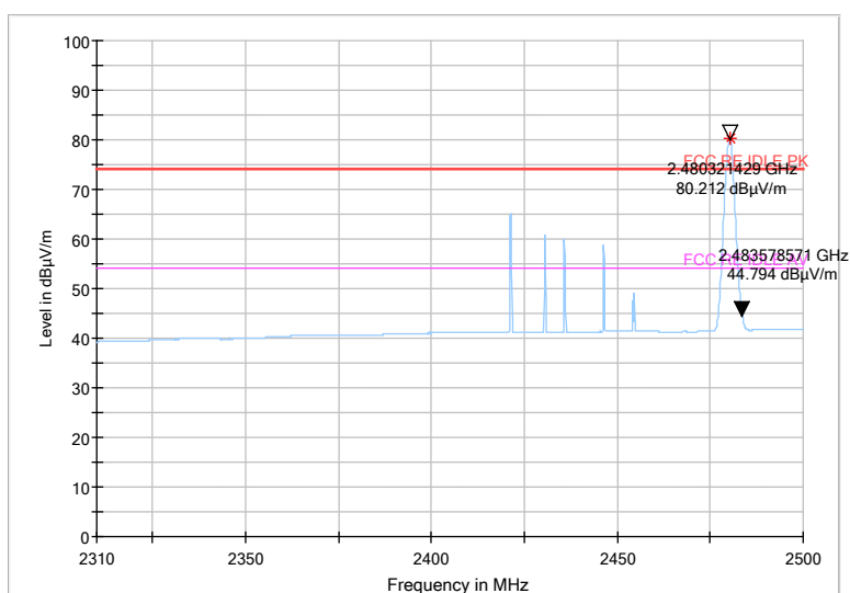
Fig.49 Radiated emission (Power): \pi/4 DQPSK, high channel
