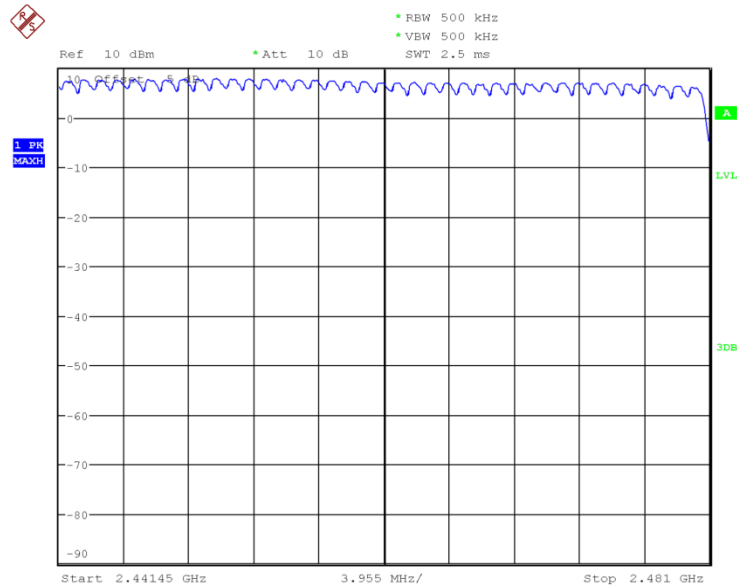
Fig.87 Number of hopping frequency: \pi/4 DQPSK, Ch0~39
