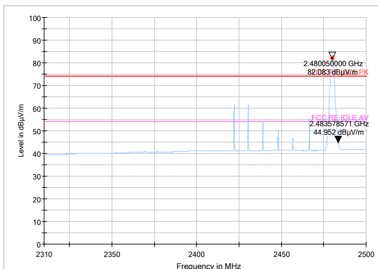
Fig.54 Radiated emission (Power): 8DPSK, high channel
