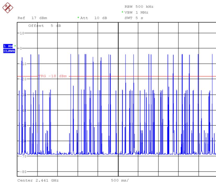
Fig.58 Number of Transmissions Measurement: Ch39, Packet DH3
