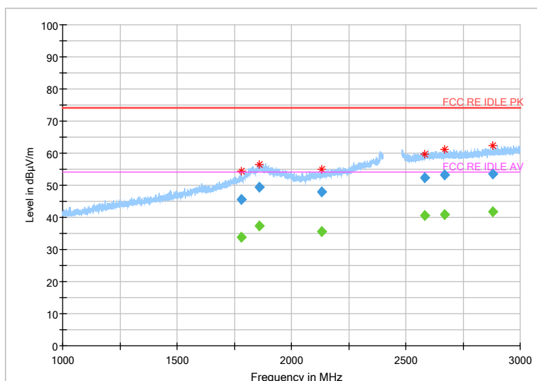
Fig.46 Radiated emission: \pi/4 DQPSK, Ch0, 1GHz~3GHz
