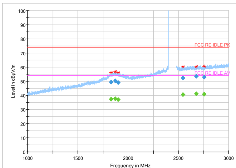
Fig.51 Radiated emission: 8DPSK, Ch0, 1GHz~3GHz
