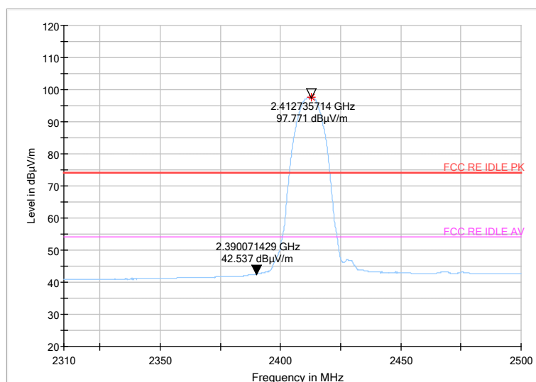
Fig 57. Radiated emission (Power): 802.11b, low channel
