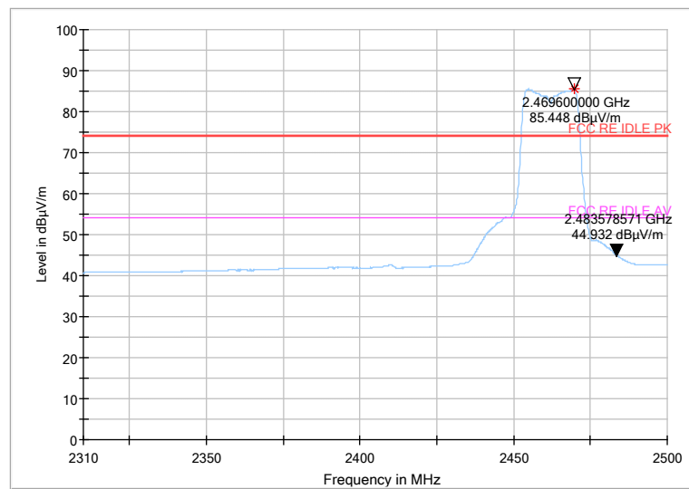
Fig 68. Radiated emission (Power): 802.11n, high channel
