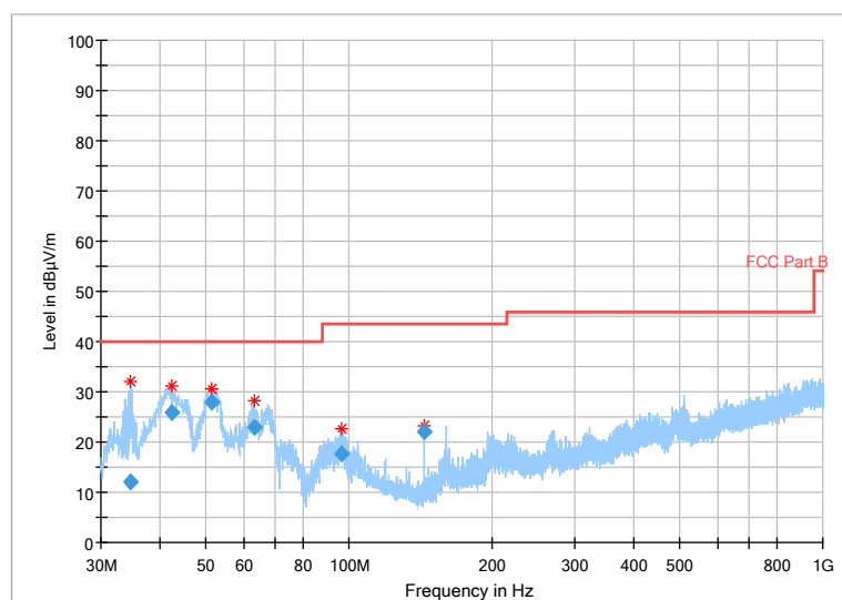
Fig 74. Radiated Spurious Emission (802.11 n-40MHz,Ch9,30MHz~1GHz)
