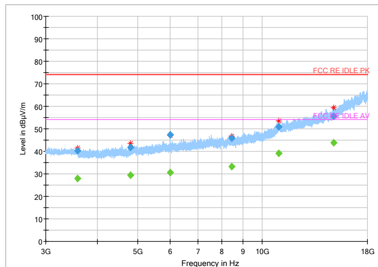
Fig 66. Radiated Spurious Emission (802.11g,Ch11,3GHz~18GHz)
