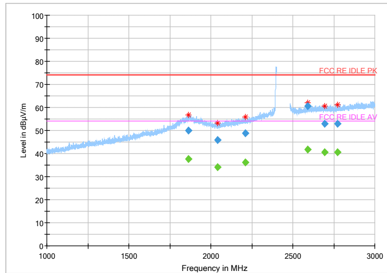
Fig 65. Radiated Spurious Emission (802.11g,Ch11,1GHz~3GHz)
