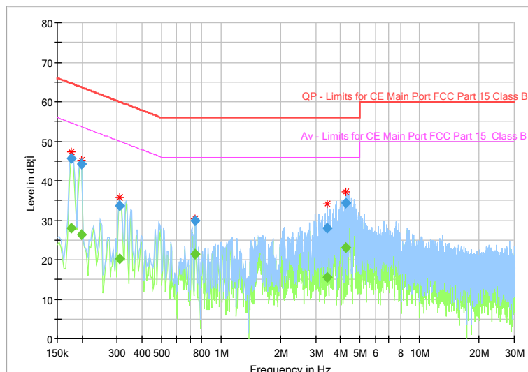
Fig.77 AC Power line Conducted Emission
