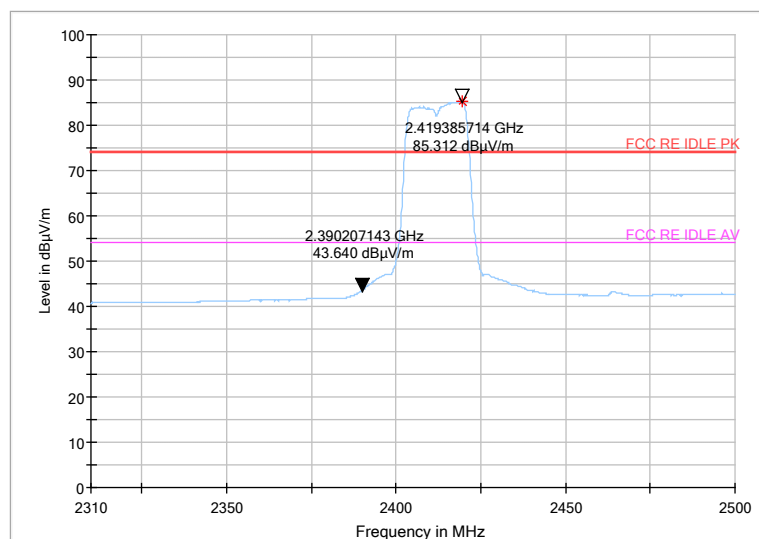
Fig 67. Radiated emission (Power): 802.11n, low channel
