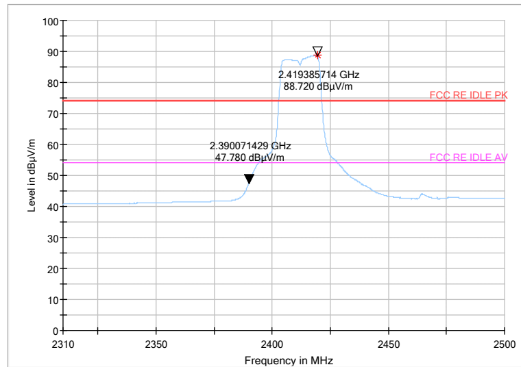
Fig 62. Radiated emission (Power): 802.11g, low channel
