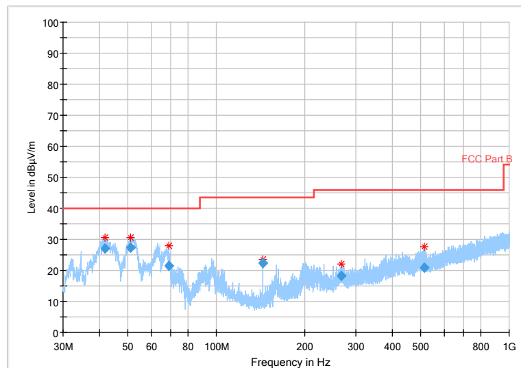
Fig 64. Radiated Spurious Emission (802.11g,Ch11,30MHz~1GHz)
