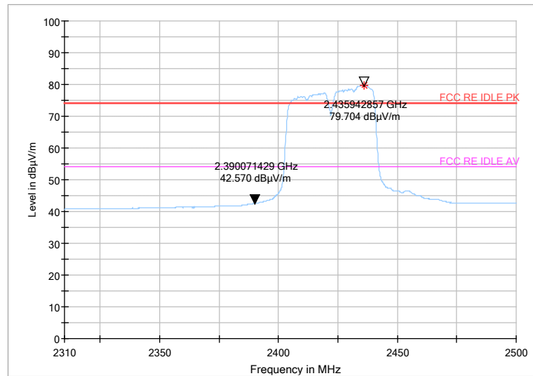
Fig 72. Radiated emission (Power): 802.11n (40M) , low channel
