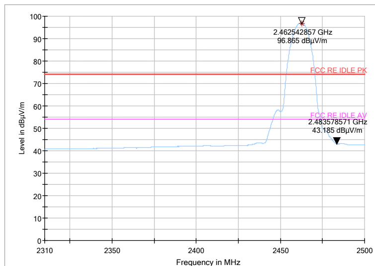
Fig 58. Radiated emission (Power): 802.11b, high channel
