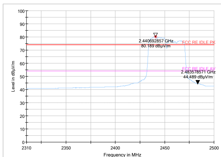
Fig 73. Radiated emission (Power): 802.11n (40M) , high channel
