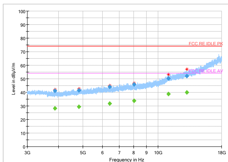
Fig 71. Radiated Spurious Emission (802.11 n-20MHz,Ch1,3GHz~18GHz)
