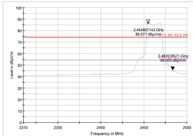
Fig 63. Radiated emission (Power): 802.11g, high channel
