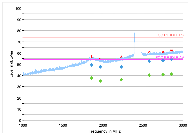
Fig 60. Radiated Spurious Emission (802.11b,Ch1,1GHz~3GHz)
