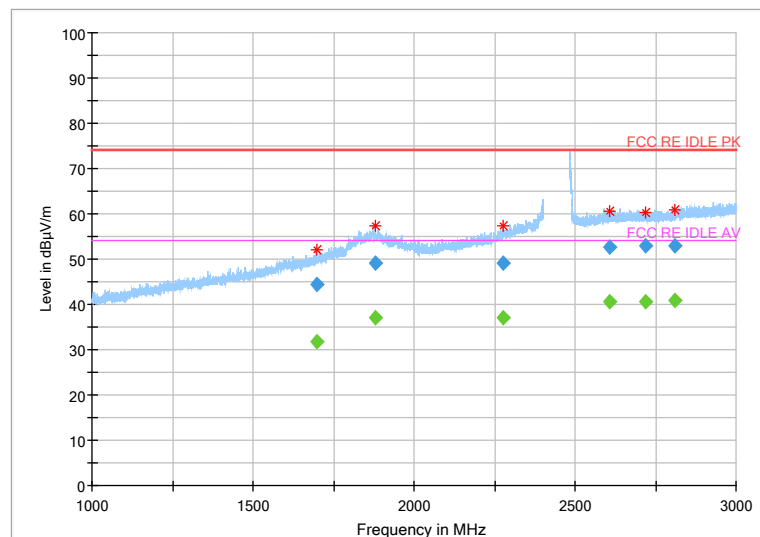
Fig 70. Radiated Spurious Emission (802.11 n-20MHz,Ch1,1GHz~3GHz)
