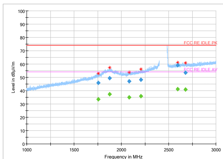
Fig 75. Radiated Spurious Emission (802.11 n-40MHz,Ch9,1GHz~3GHz)
