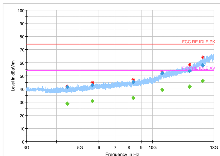
Fig 76. Radiated Spurious Emission (802.11 n-40MHz,Ch9,3GHz~18GHz)
