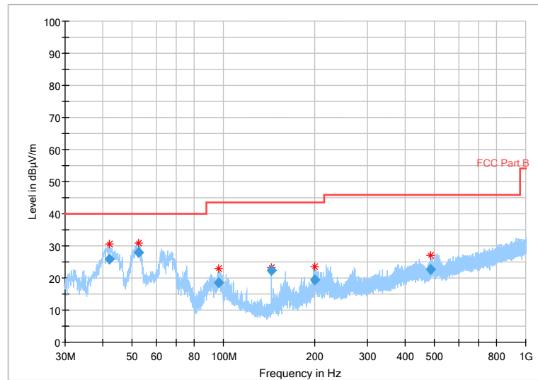
Fig 59. Radiated Spurious Emission (802.11b,Ch1,30MHz~1GHz)
