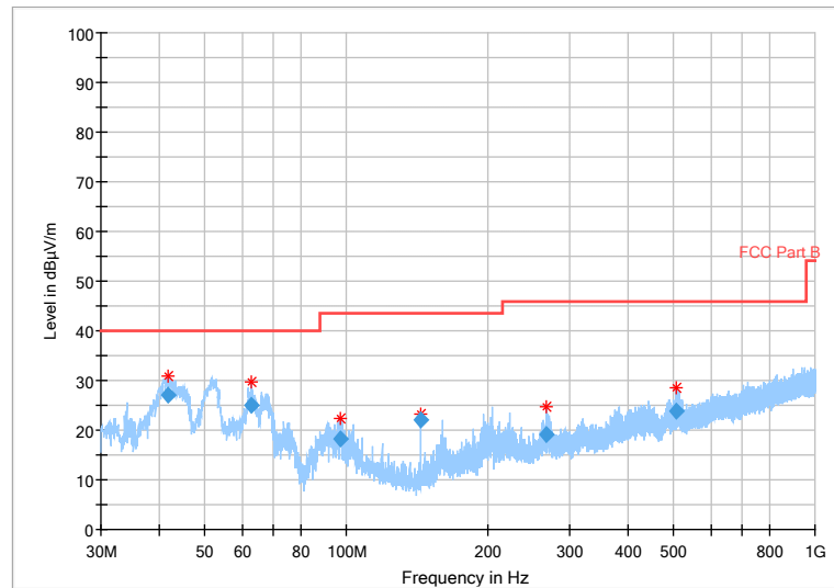
Fig 69. Radiated Spurious Emission (802.11 n-20MHz,Ch1,30MHz~1GHz)
