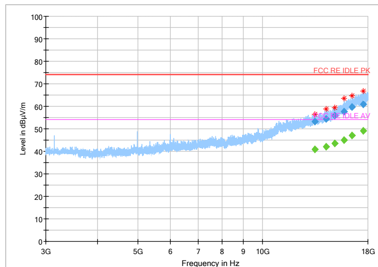
Fig 61. Radiated Spurious Emission (802.11b,Ch1,3GHz~18GHz)
