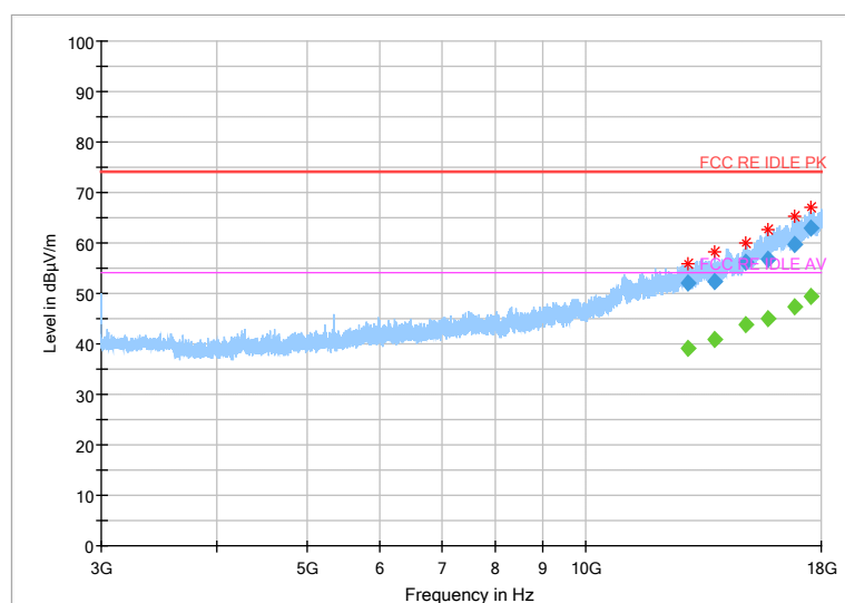
Fig 66. Radiated Spurious Emission (802.11g, Ch11, 3GHz~18GHz)
