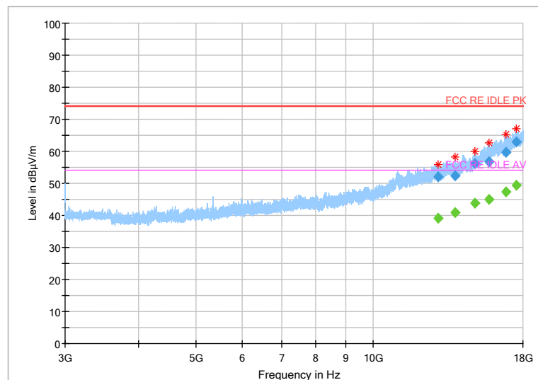
Fig 71. Radiated Spurious Emission (802.11 n-20MHz,Ch1,3GHz~18GHz)
