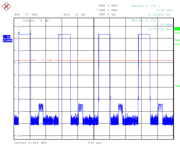
Fig.66 Number of Transmissions Measurement: Ch39, Packet 2-DH5
