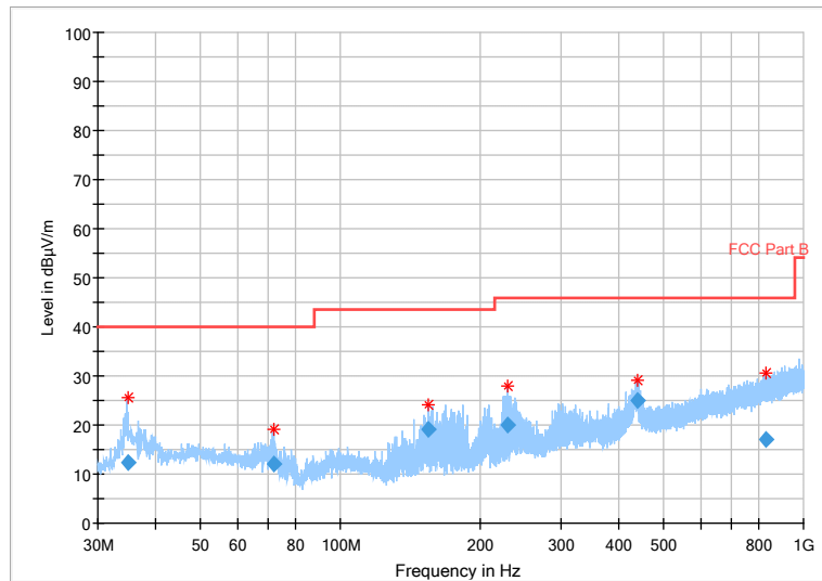
Fig 45 Radiated emission: \pi/4 DQPSK, Ch0, 30MHz~1GHz
