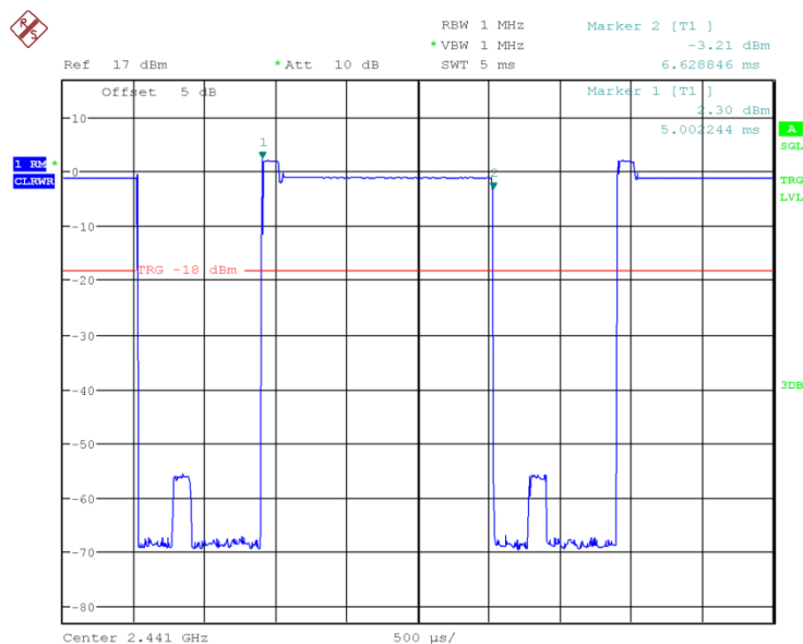
Fig.68 Number of Transmissions Measurement: Ch39, Packet 3-DH1
