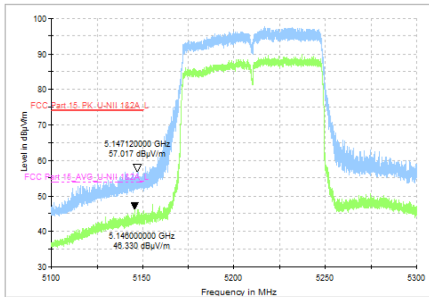
Fig. 61 Band Edges (802.11ac-VHT80, CH42 5210MHz)
