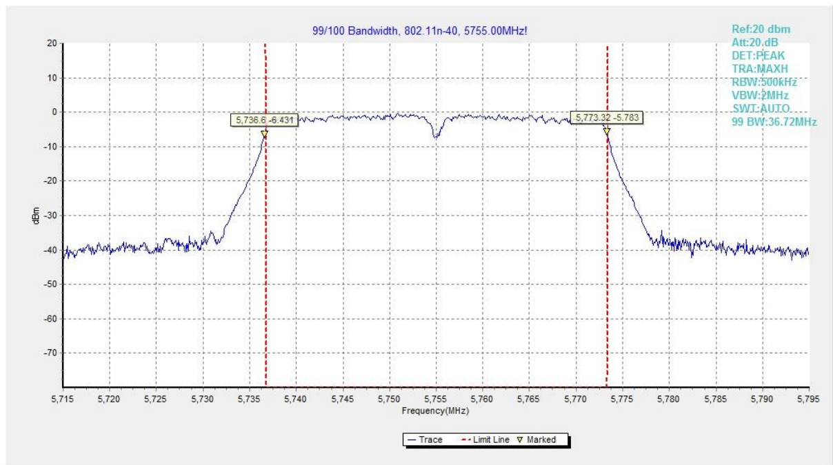
Fig. 43 99% Occupied Bandwidth (802.11n-HT40, 5755MHz)
