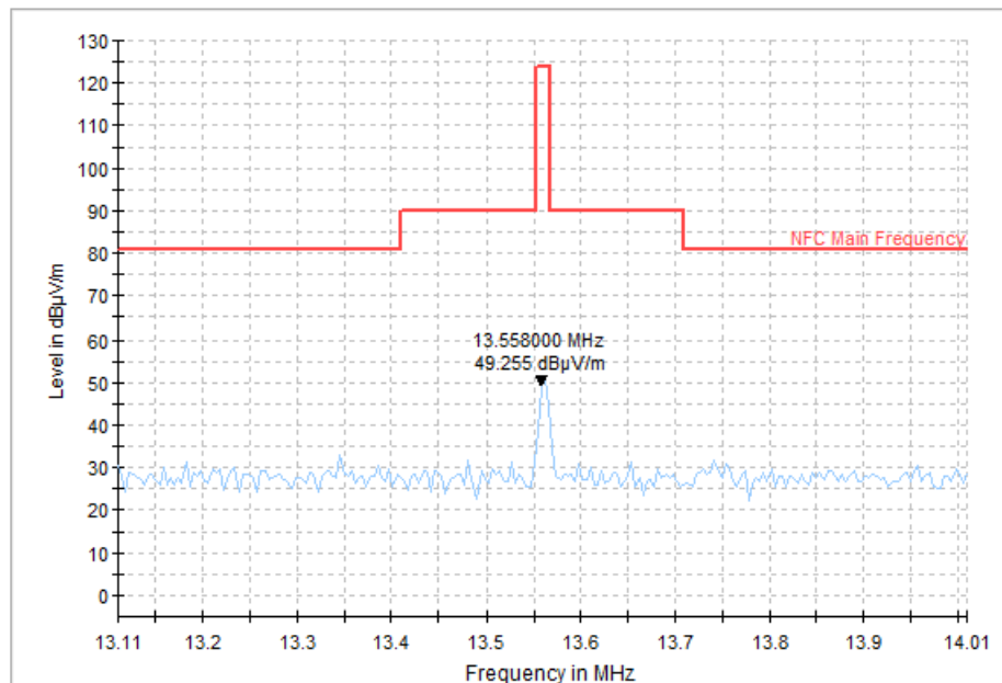
Figure A-1 Electric Field Strength
