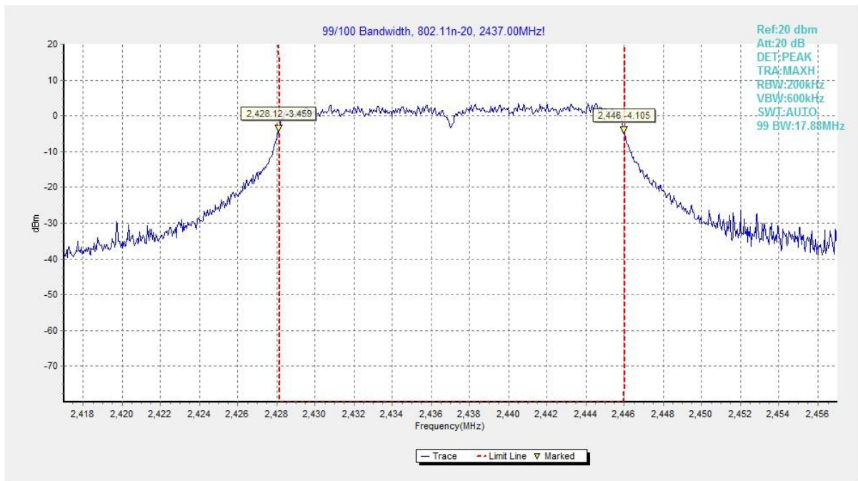
Fig.77 99% Occupied Bandwidth (802.11n HT20, CH 6)
