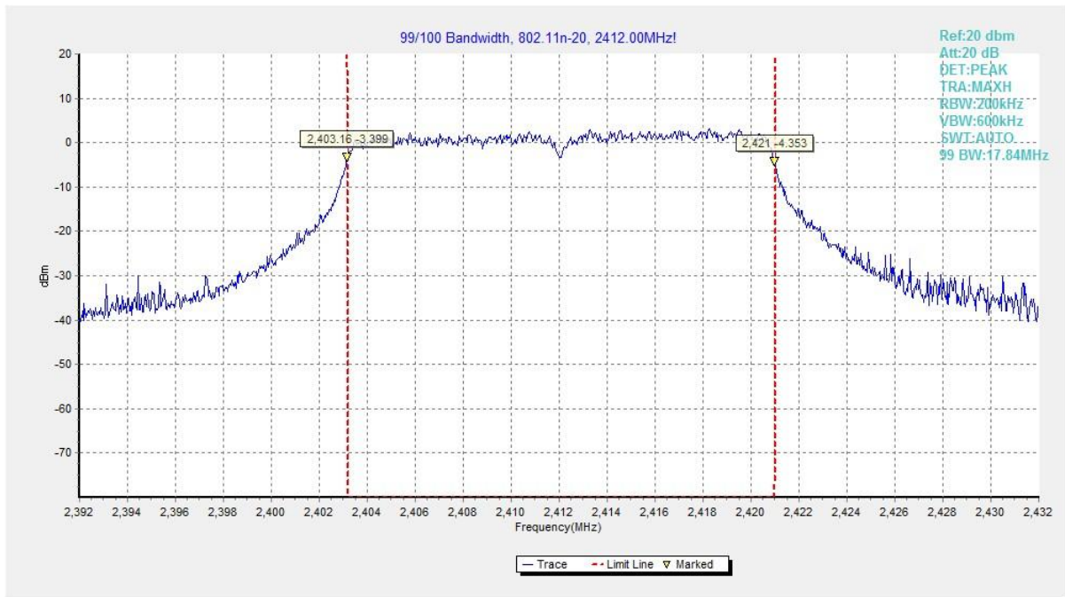
Fig.76 99% Occupied Bandwidth (802.11n HT20, CH 1)
