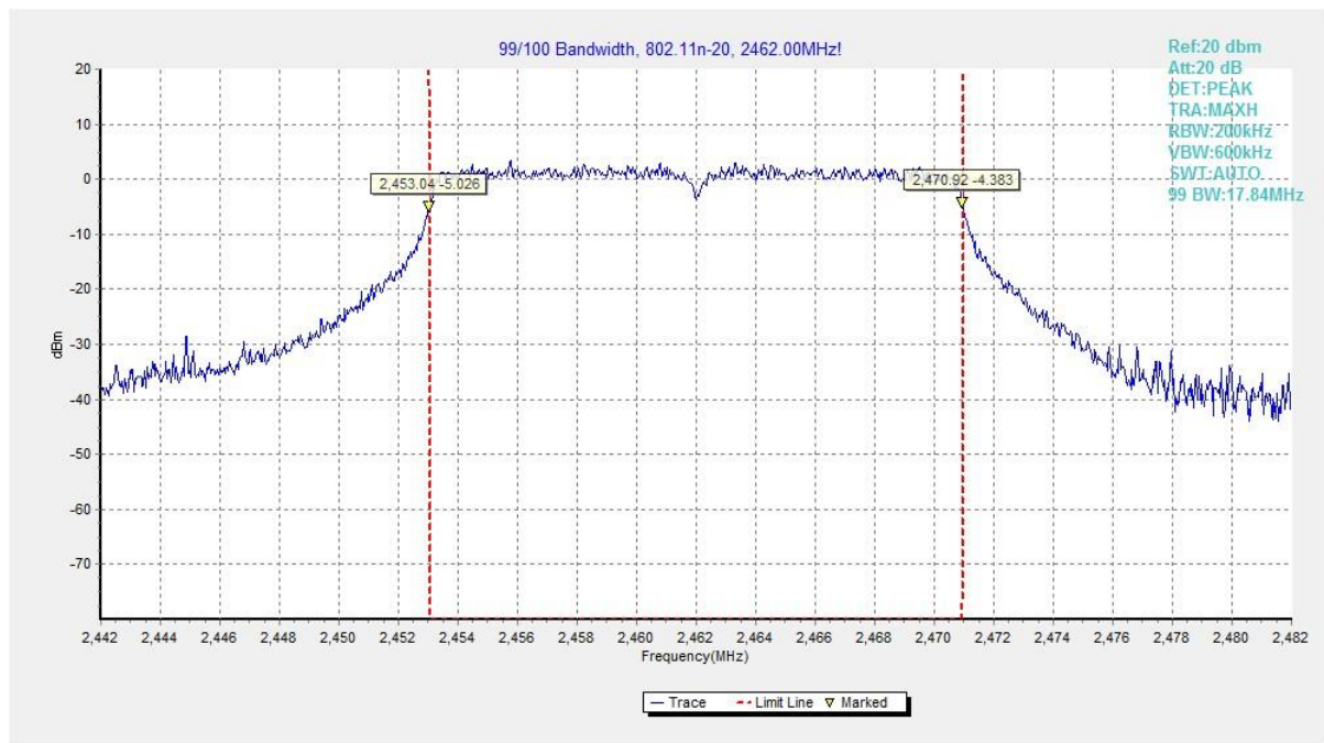
Fig.78 99% Occupied Bandwidth (802.11n HT20, CH 11)
