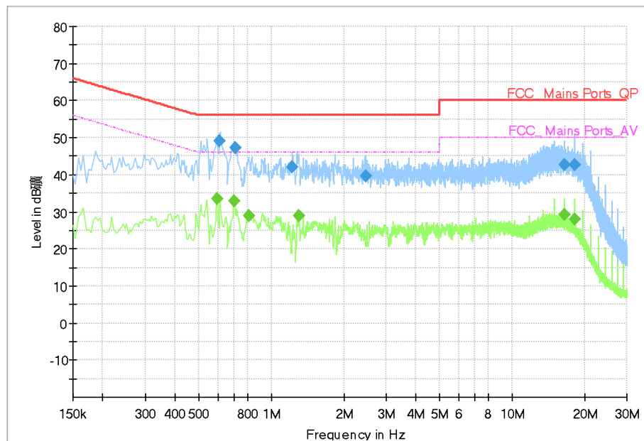
Fig.69 AC Power line Conducted Emission (Idle, 120V)
