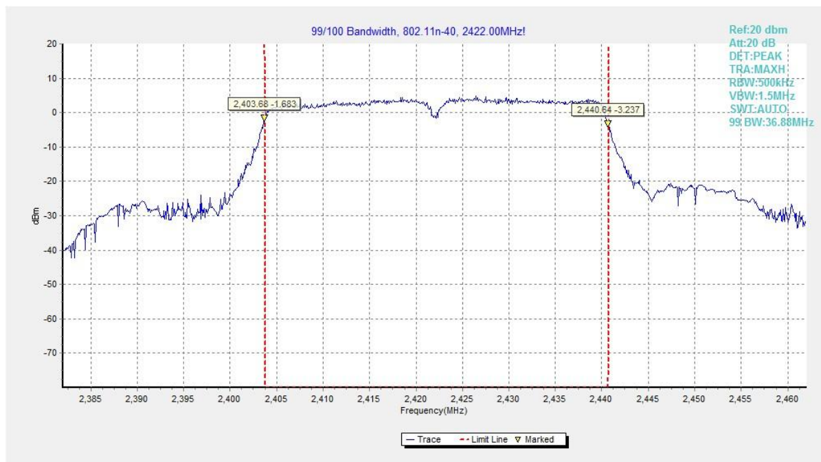
Fig.79 99% Occupied Bandwidth (802.11n HT40, CH 3)
