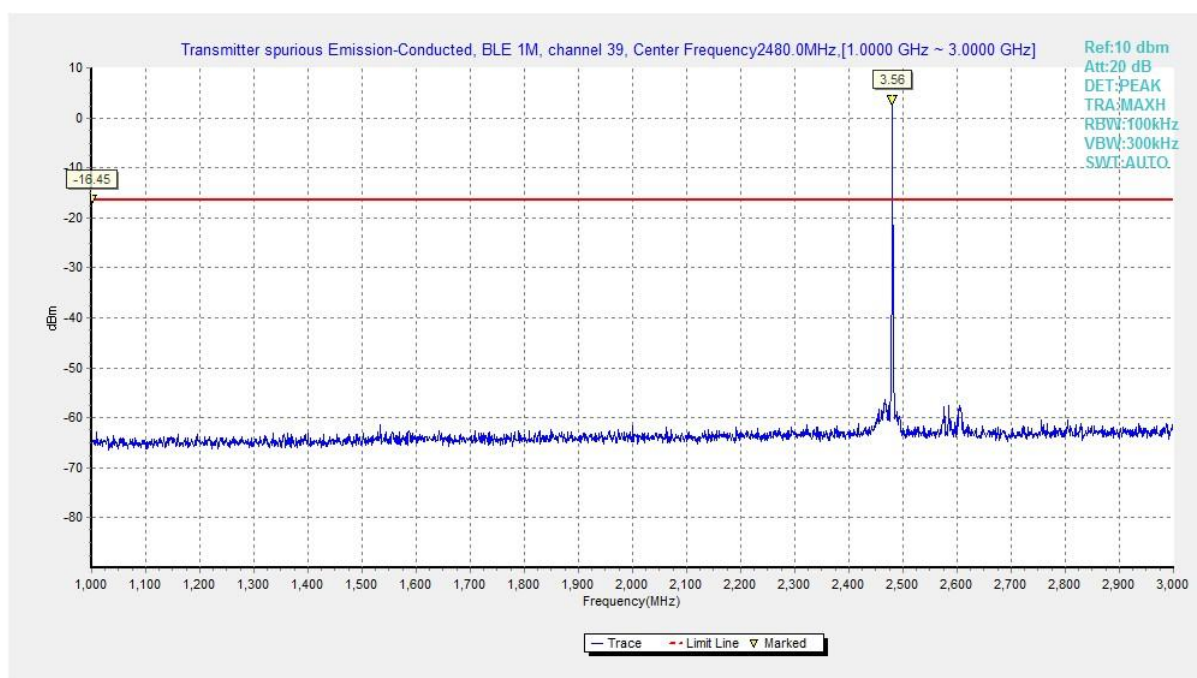
Fig.13 Conducted Spurious Emission (Ch39, 1 GHz-3 GHz), LE 1M
