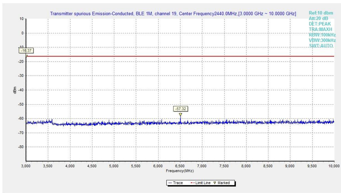
Fig.12 Conducted Spurious Emission (Ch19, 3 GHz-10 GHz), LE 1M
