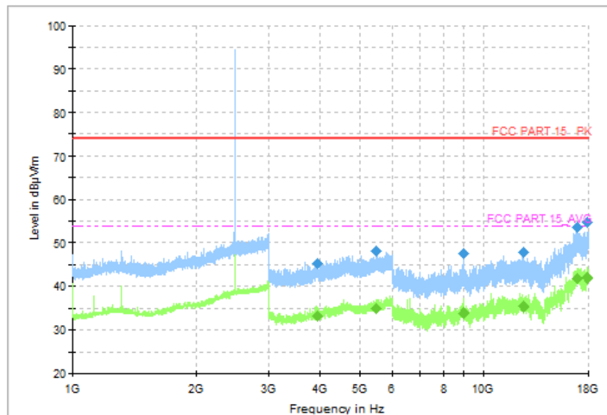
Fig.22 Radiated Spurious Emission (Ch39, 1 GHz - 18 GHz), 1M
