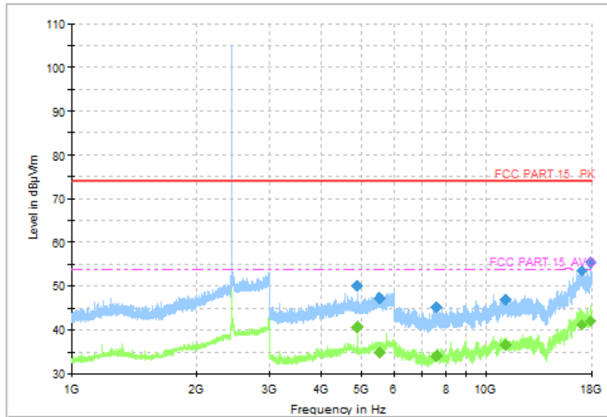
Fig. 39 Radiated Spurious Emission ( \pi/4 DQPSK, Ch39, 1GHz ~ 18GHz)
