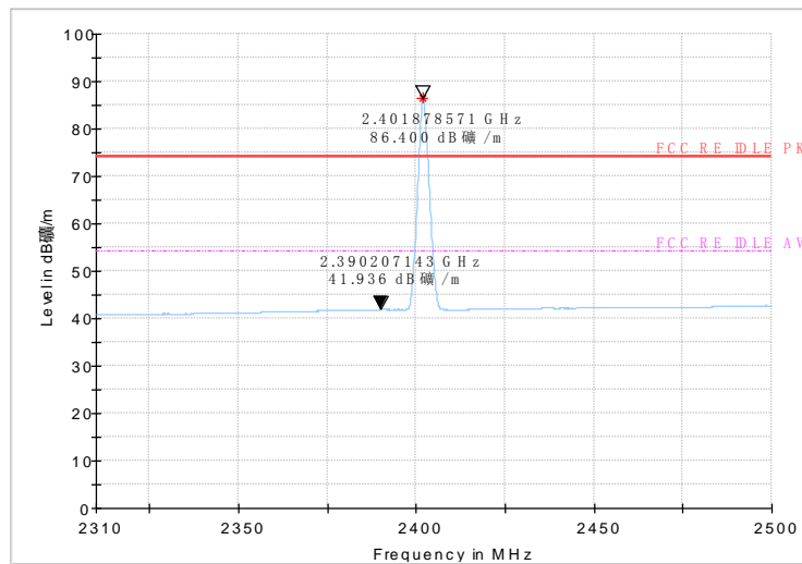
Fig 9 Radiated emission (Power): \pi/4 DQPSK, low channel
