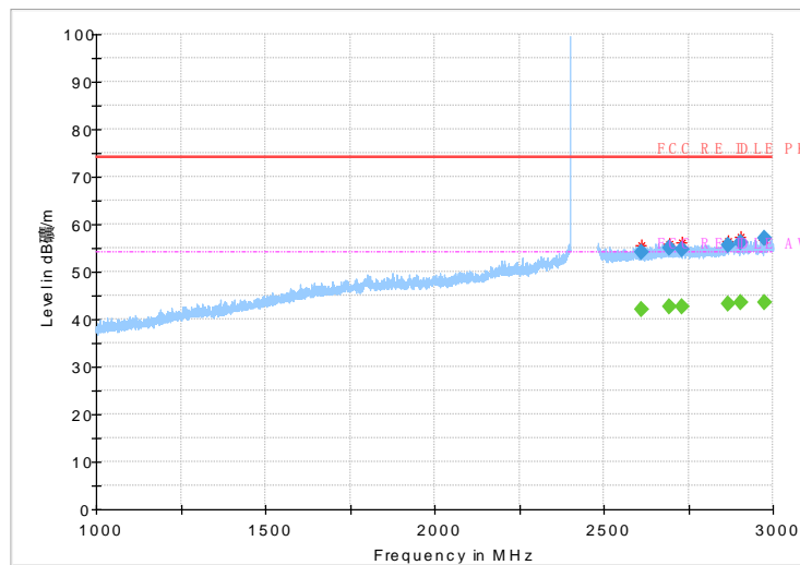
Fig 12 Radiated emission: 8DPSK, Ch0, 1GHz~3GHz
