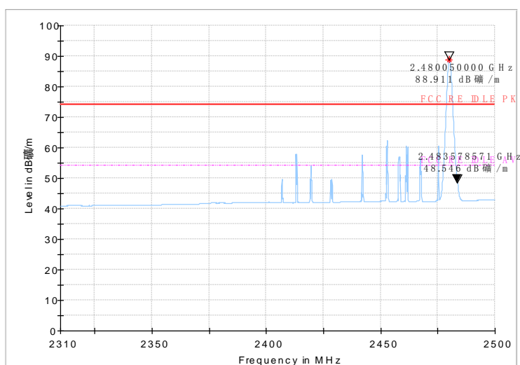
Fig 5 Radiated emission (Power): GFSK, high channel
