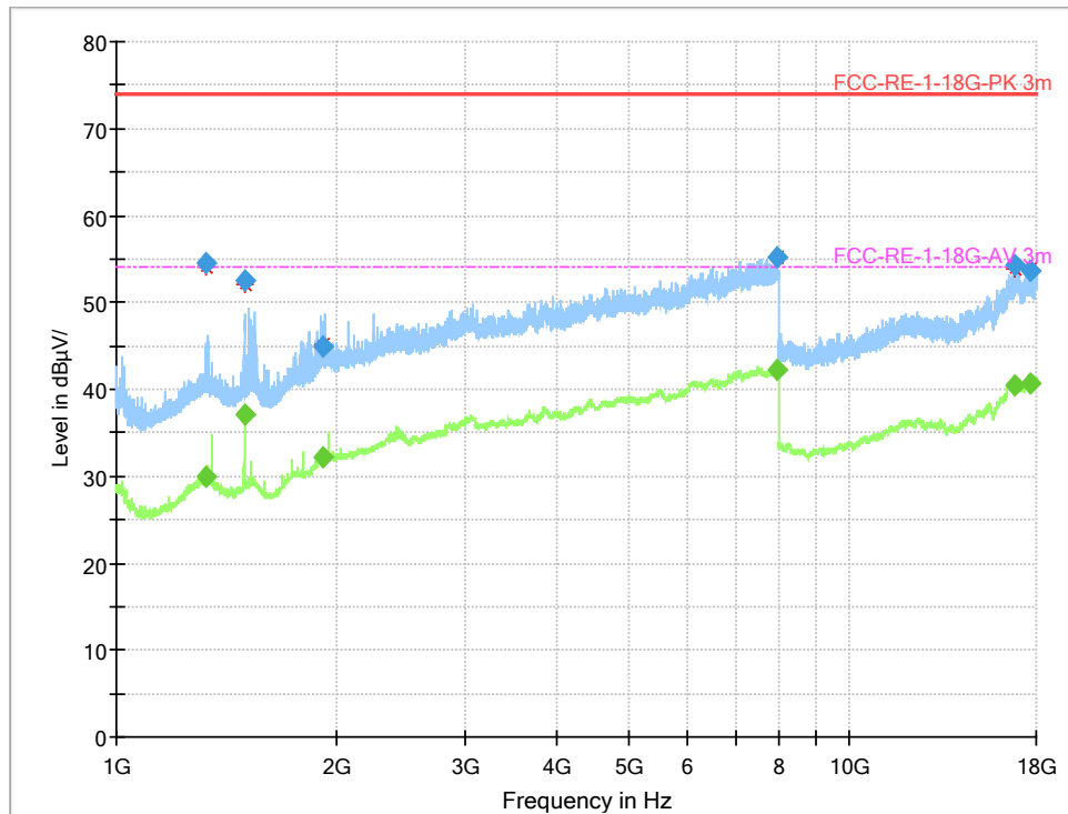
Figure A.1-3 Mode 6 (1GHz-18GHz)-V
