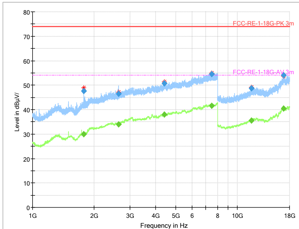
Figure A.1-2 Mode 6 (1GHz-18GHz)-H
