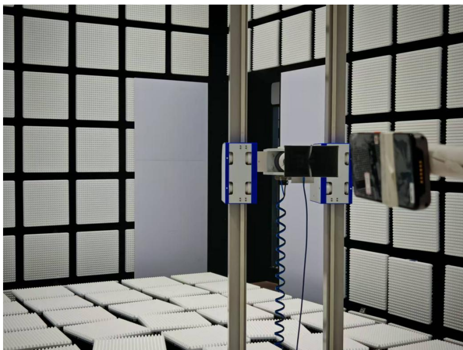
Description: Radiated Emissions above 1GHz Test Setup
