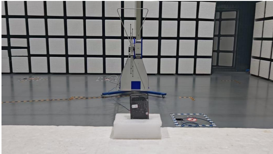
Description: Radiated Emissions below 1GHz Test Setup
