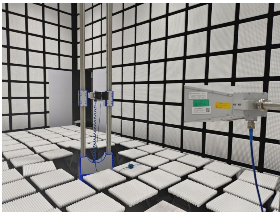
Description: substitution Antenna for Radiated Emissions above 1GHz Test Setup
