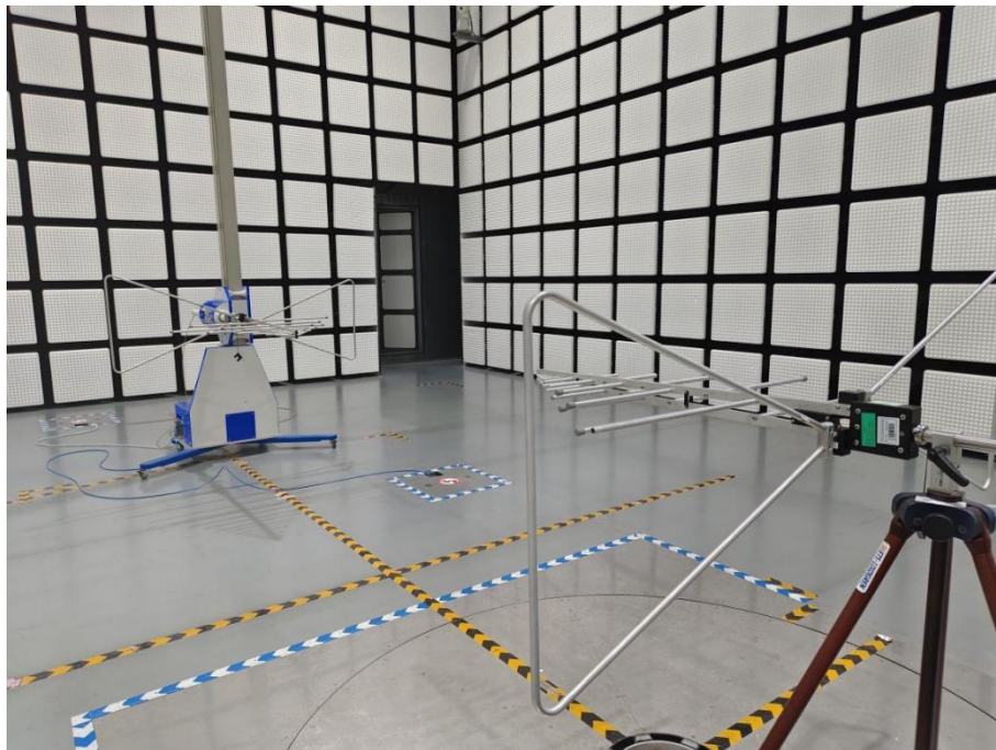
Description: substitution Antenna for Radiated Emissions below 1GHz Test Setup
