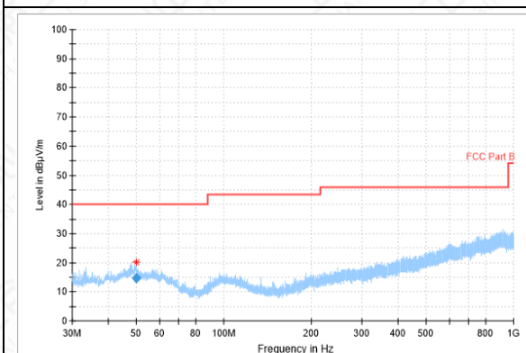
RSE-11N-CH100-30MHz-1GHz
