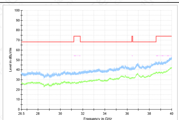
RSE-11N-CH56-26.5GHz-40GHz
