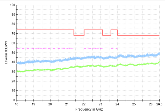
RSE-11N(40M)-CH54-18GHz-26.5GHz
