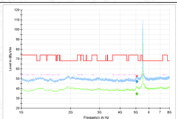
RSE-11N-CH100-1GHz-8GHz
