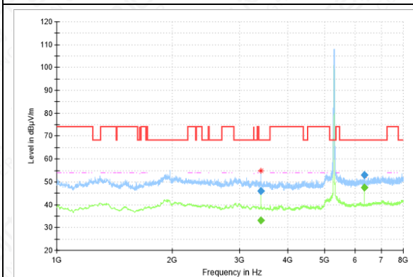
RSE-11N-CH56-1GHz-8GHz
