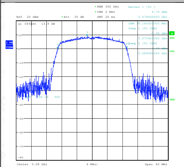
11AC20SISO-Ant1-5580
