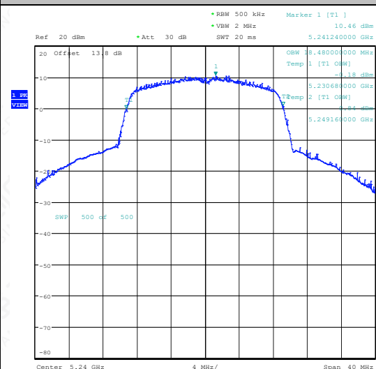
11N20SISO-Ant1-5240
