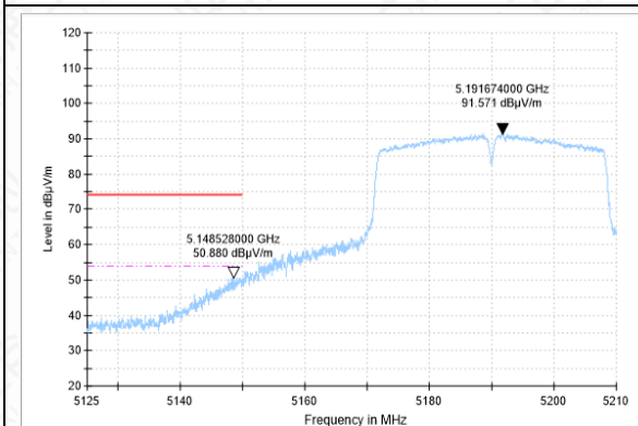
BANDEGE-11N(40M)-CH38-AV-16
