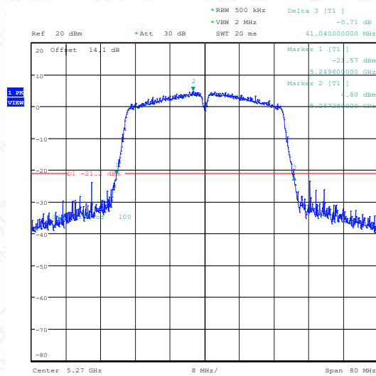
11AC40SISO-Ant1-5270
