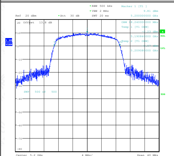
11AC20SISO-Ant1-5200
