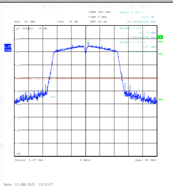
11AC40SISO-Ant1-5670
