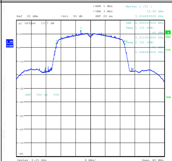
11N40SISO-Ant1-5230
