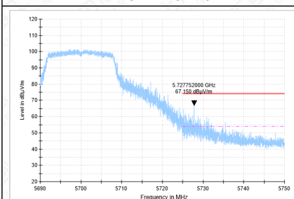
BANEDGE-11A-CH140-PK
