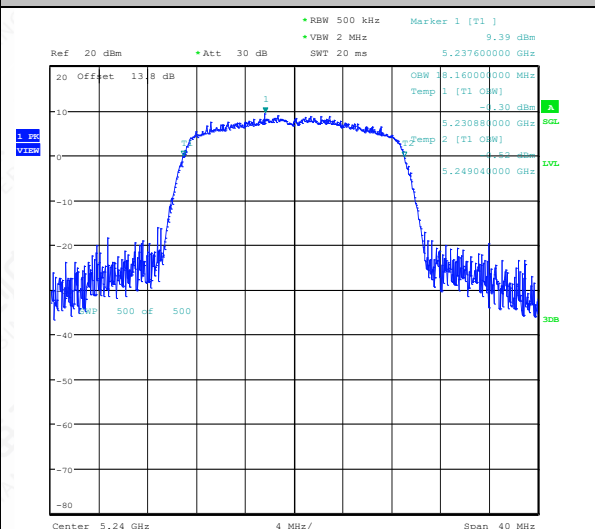
11AC20SISO-Ant1-5240
