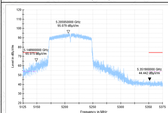
BANDEDGE-11AC(80M)-CH42-PK
