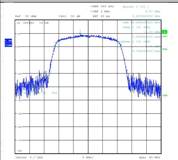
11AC20SISO-Ant1-5700
