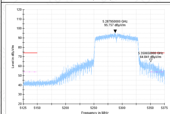
BANDEDGE-11AC(80M)-CH58-PK
