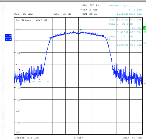
11AC20SISO-Ant1-5500
