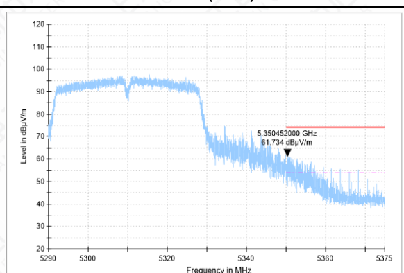
BANDEGE-11N(40M)-CH62-PK
