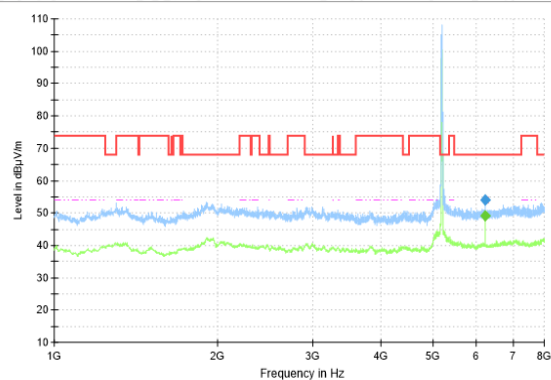
RSE-11AC-CH36-1GHz-8GHz
