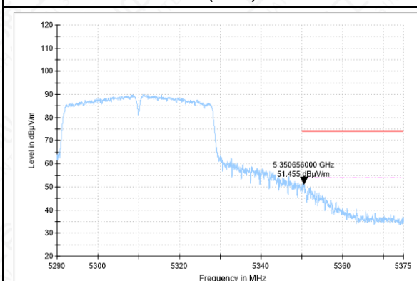
BANDEGE-11N(40M)-CH62-AV-17
