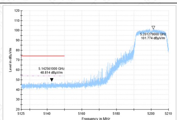
BANEDGE-11N-CH40-PK
