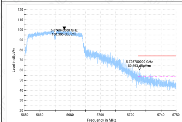
BANDEDGE-11AC(40M)-CH134-PK
