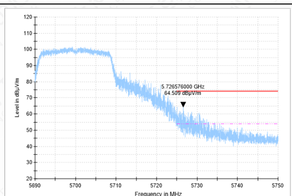
BANDEGE-11N-CH140-PK
