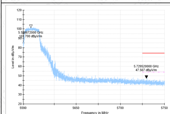
BANEDGE-11A-CH120-PK
