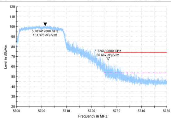
BANDEGE-11AC-CH140-PK
