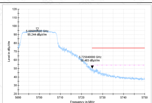
BANEDGE-11A-CH140-AV
