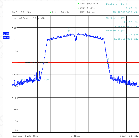
11AC40SISO-Ant1-5310
