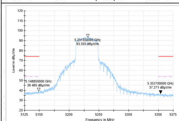
BANDEGE-11N(40M)-CH46-AV
