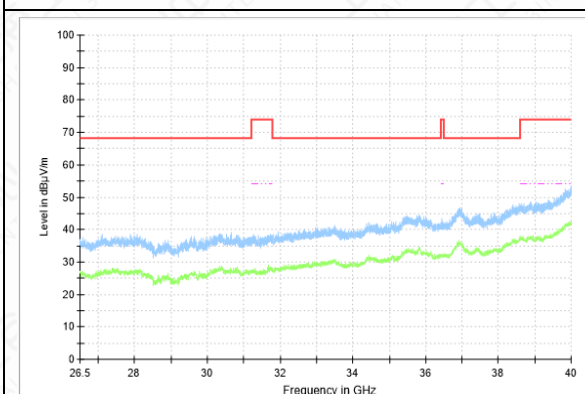
RSE-11N-CH36-26.5GHz-40GHz
