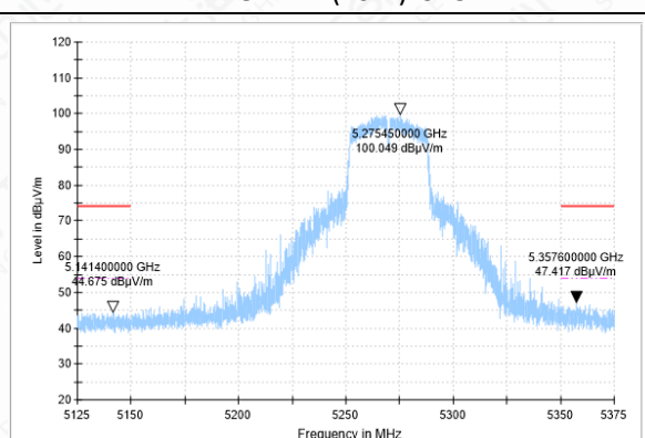
BANDEGE-11N(40M)-CH54-PK
