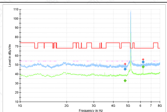
RSE-11N-CH36-1GHz-8GHz
