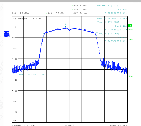
11AC40SISO-Ant1-5230
