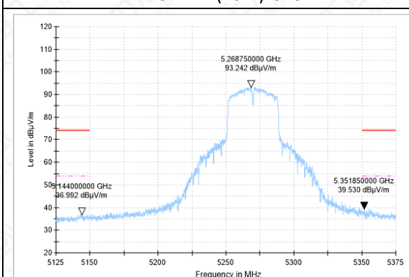
BANDEGE-11N(40M)-CH54-AV
