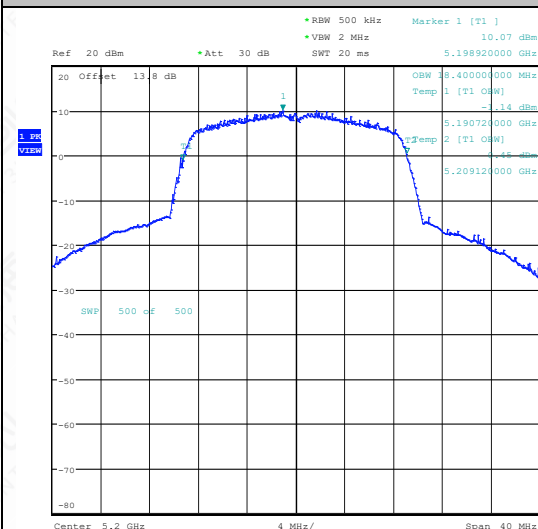
11N20SISO-Ant1-5200
