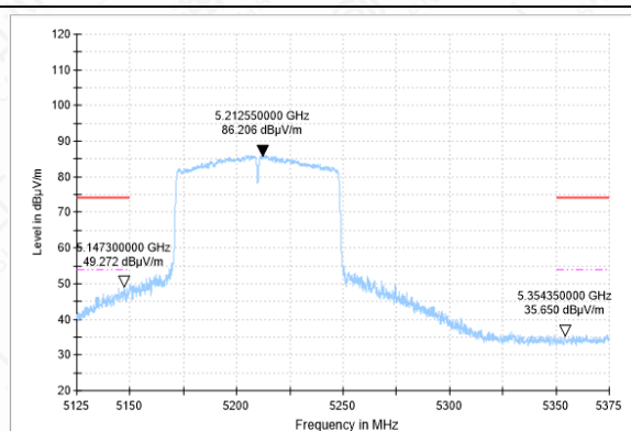
BANDEDGE-11AC(80M)-CH42-AV-14
