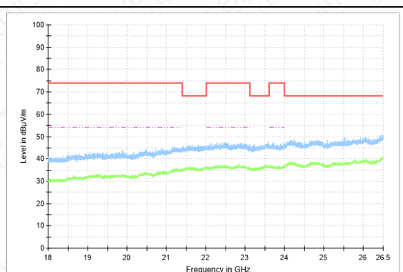
RSE-11N-CH36-18GHz-26.5GHz
