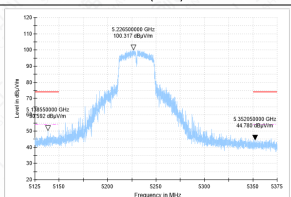
BANDEGE-11N(40M)-CH46-PK
