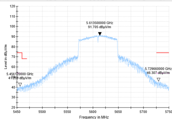
BANDEGE-11AC(80M)-CH122-AV
