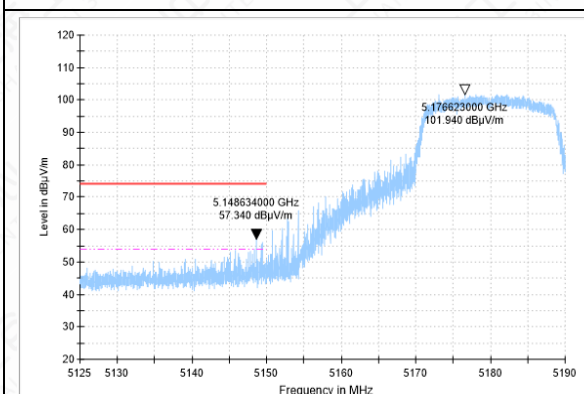
BANEDGE-11N-CH36-PK
