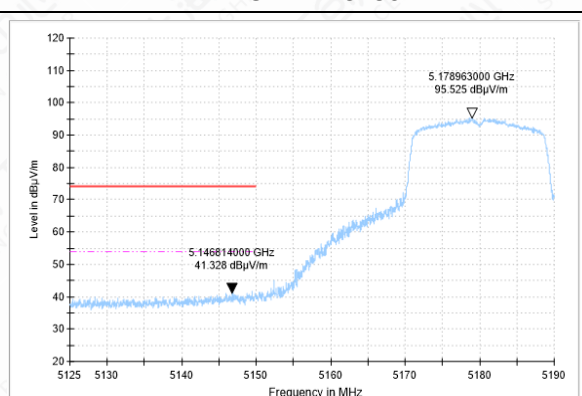
BANEDGE-11N-CH36-AV
