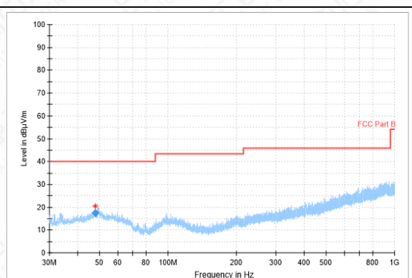
RSE-11N-CH56-30MHz-1GHz
