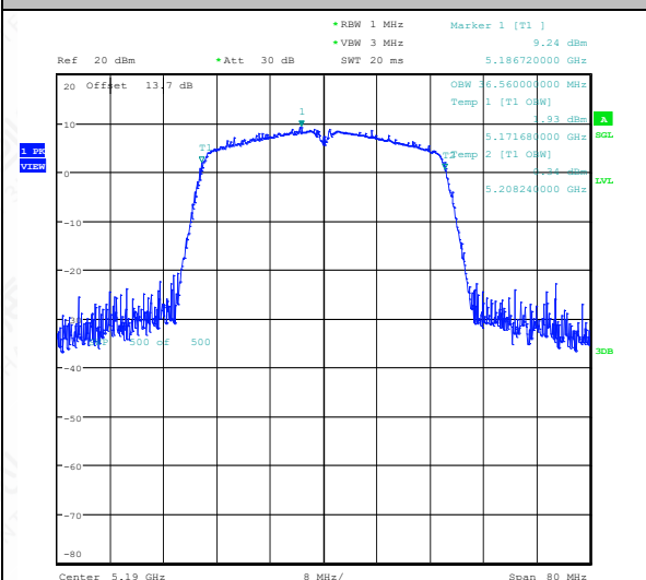
11AC40SISO-Ant1-5190
