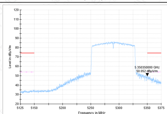
BANDEDGE-11AC(80M)-CH58-AV-14
