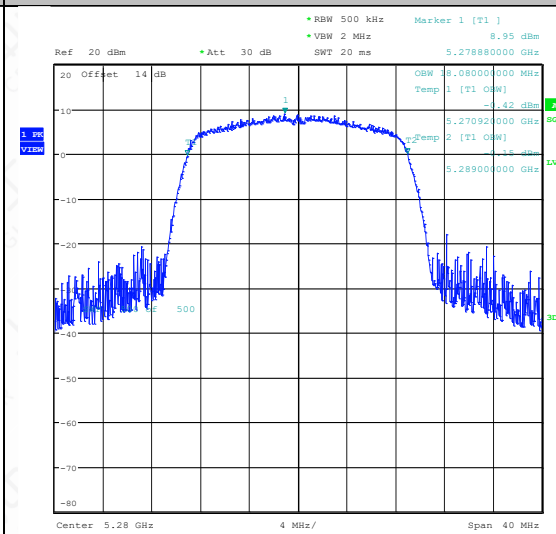
11AC20SISO-Ant1-5280
