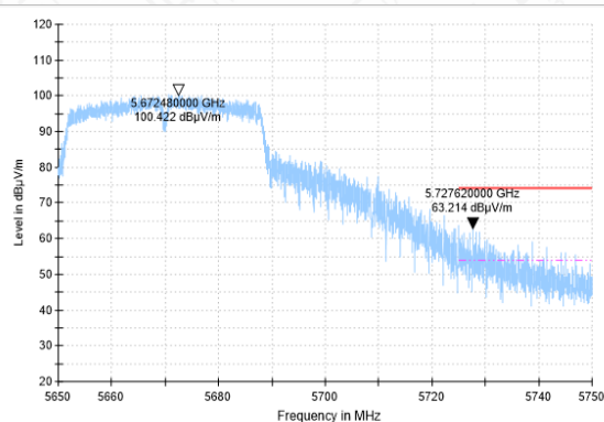
BANDEGE-11N(40M)-CH134-PK
