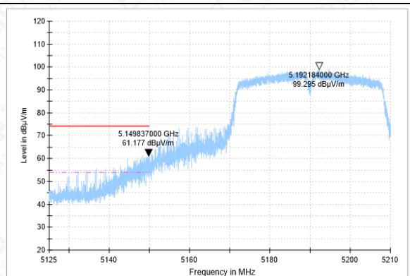
BANDEGE-11N(40M)-CH38-PK
