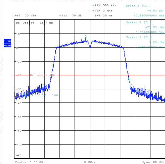
11AC40SISO-Ant1-5550
