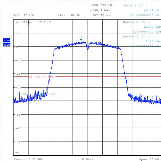
11AC40SISO-Ant1-5510
