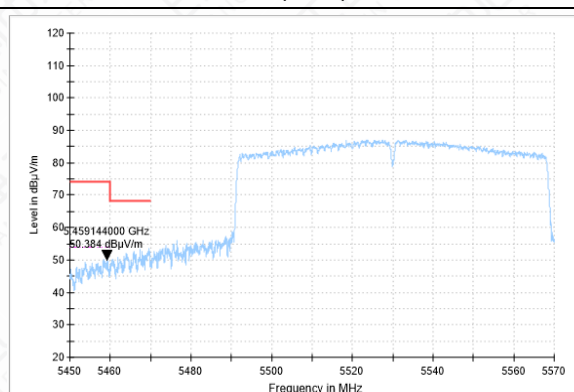
BANDEDGE-11AC(80M)-CH106-AV-14
