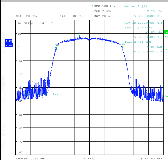
11AC20SISO-Ant1-5320
