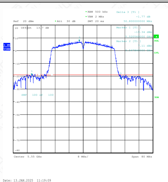
11N40SISO-Ant1-5550
