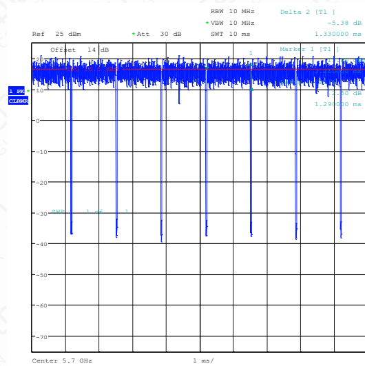
NTNV-11N20SISO-Ant1-5700
