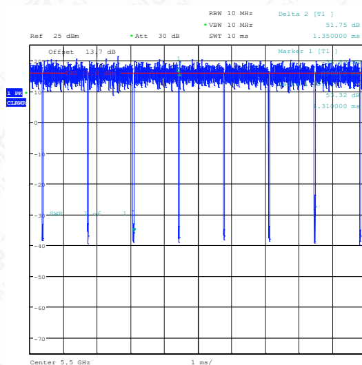
NTNV-11AC20SISO-Ant1-5500
