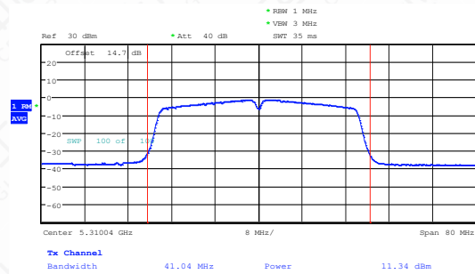
11N40SISO-Ant1-5310-PASS
