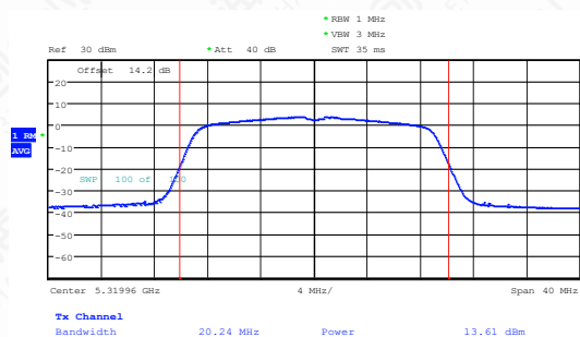
11AC20SISO-Ant1-5320-PASS
