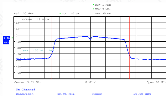
11N40SISO-Ant1-5510-PASS
