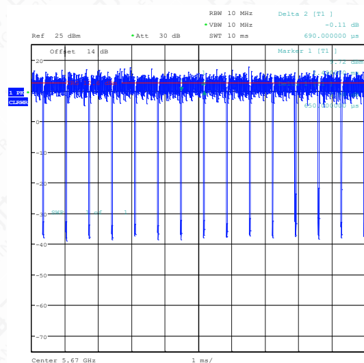
NTNV-11AC40SISO-Ant1-5670
