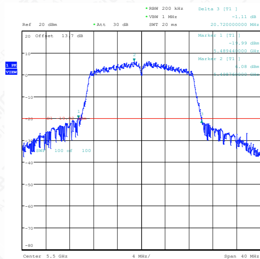
11N20SISO-Ant1-5500
