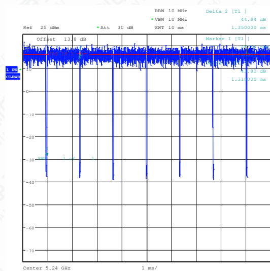
NTNV-11AC20SISO-Ant1-5240
