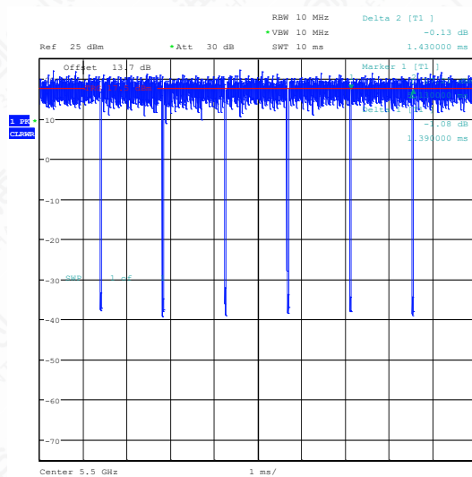
NTNV-11A-Ant1-5500
