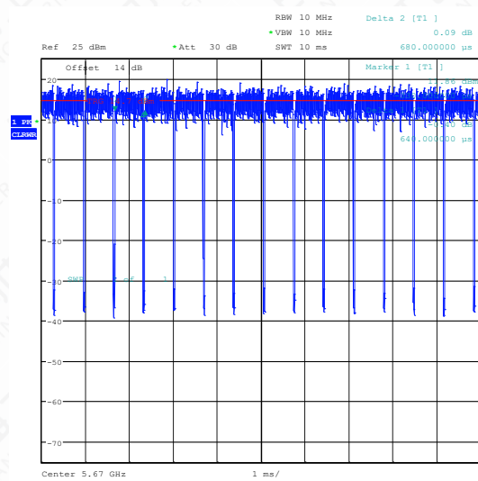
NTNV-11N40SISO-Ant1-5670
