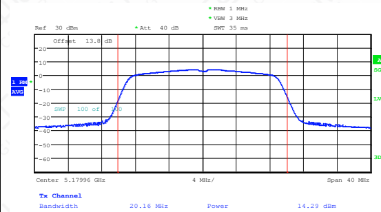
11AC20SISO-Ant1-5180-PASS
