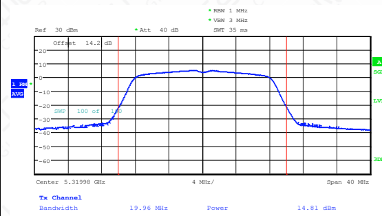
11A-Ant1-5320-PASS
