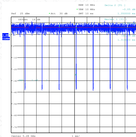
NTNV-11AC20SISO-Ant1-5280
