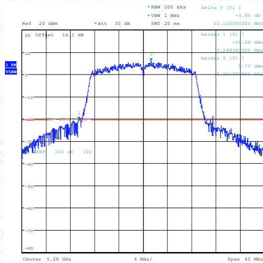
11N20SISO-Ant1-5260
