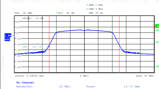
11A-Ant1-5580-PASS
