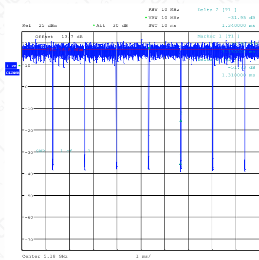
NTNV-11AC20SISO-Ant1-5180
