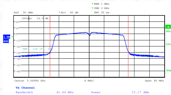
11N40SISO-Ant1-5670-PASS
