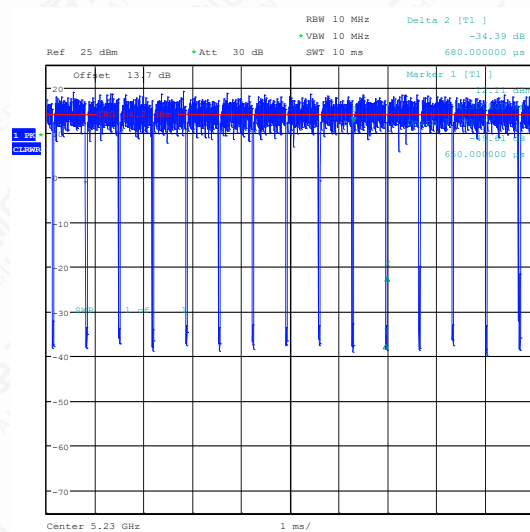
NTNV-11N40SISO-Ant1-5230
