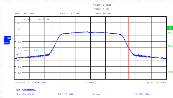
11A-Ant1-5280-PASS
