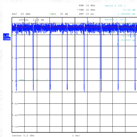
NTNV-11AC20SISO-Ant1-5200
