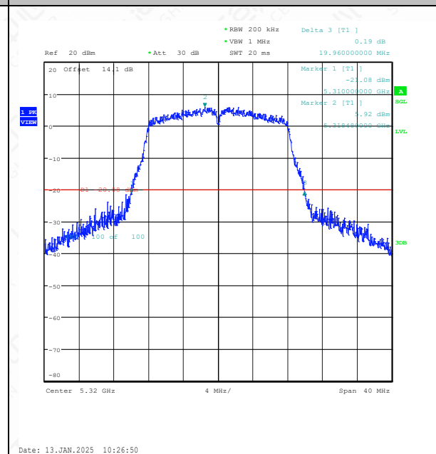
11A-Ant1-5320
