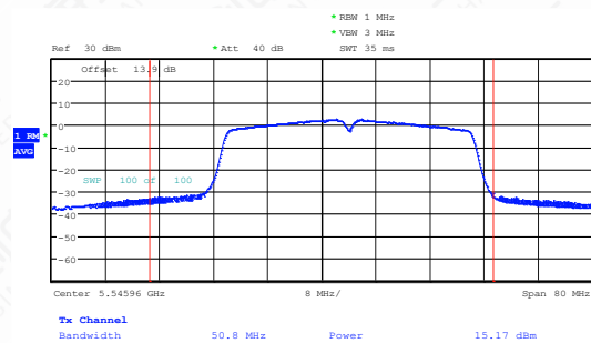
11N40SISO-Ant1-5550-PASS
