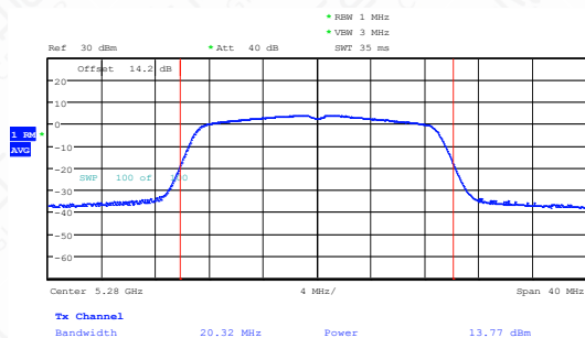
11AC20SISO-Ant1-5280-PASS
