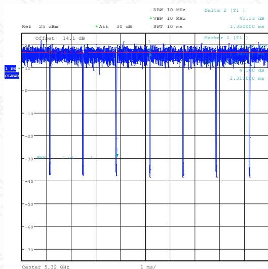
NTNV-11AC20SISO-Ant1-5320
