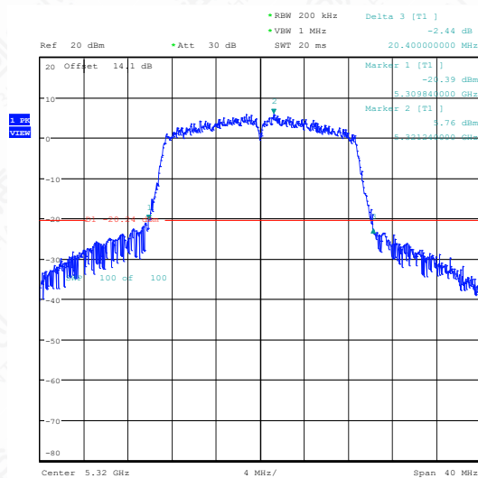
11N20SISO-Ant1-5320
