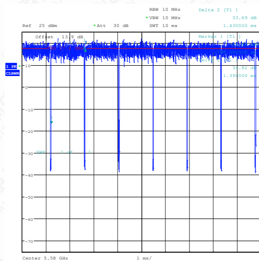
NTNV-11A-Ant1-5580
