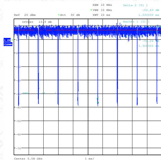
NTNV-11N20SISO-Ant1-5580
