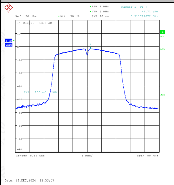
11N40SISO-Ant1-5510-PASS
