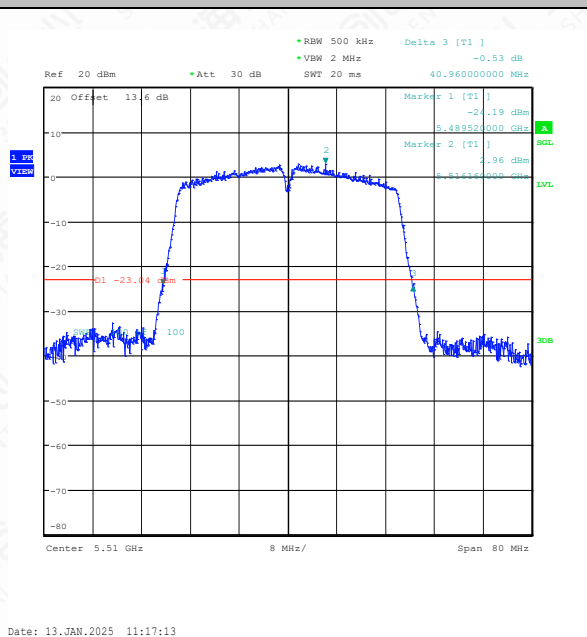
11N40SISO-Ant1-5510
