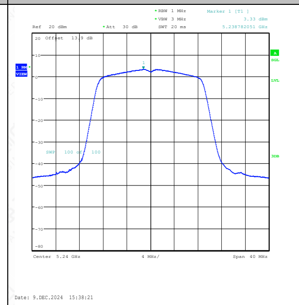
11AC20SISO-Ant1-5240-PASS
