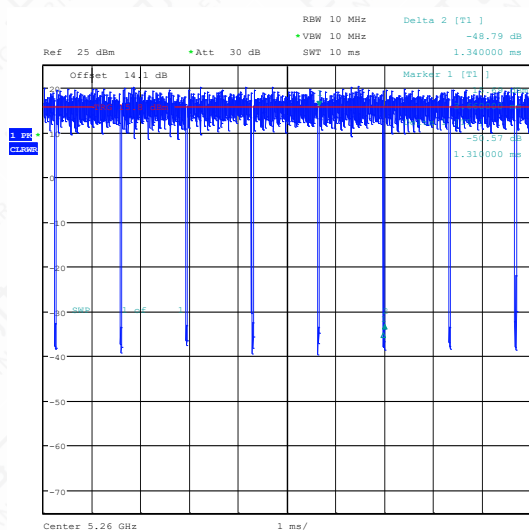
NTNV-11AC20SISO-Ant1-5260
