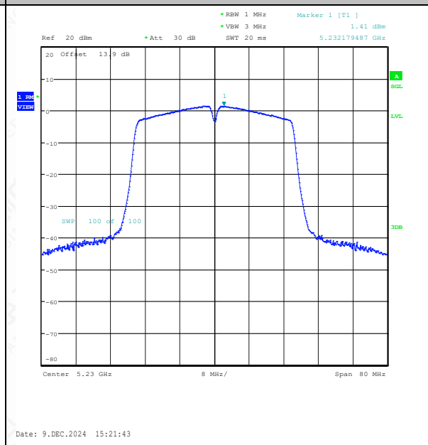
11N40SISO-Ant1-5230-PASS
