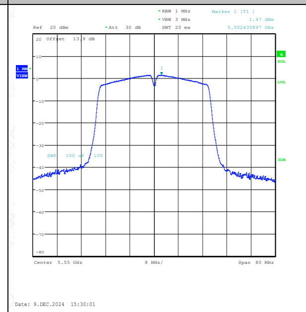
11N40SISO-Ant1-5550-PASS
