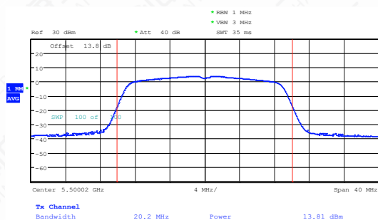
11AC20SISO-Ant1-5500-PASS
