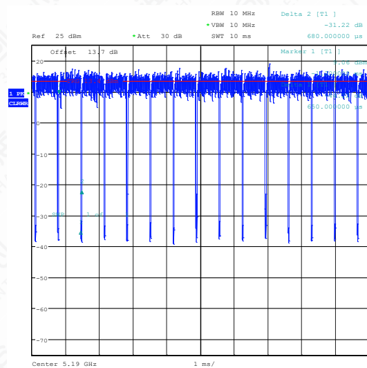
NTNV-11N40SISO-Ant1-5190
