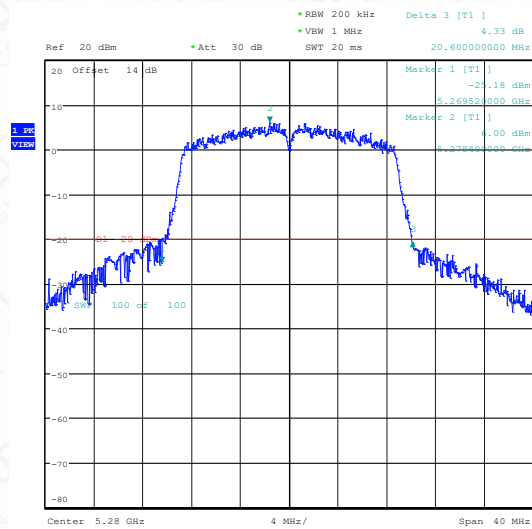
11N20SISO-Ant1-5280
