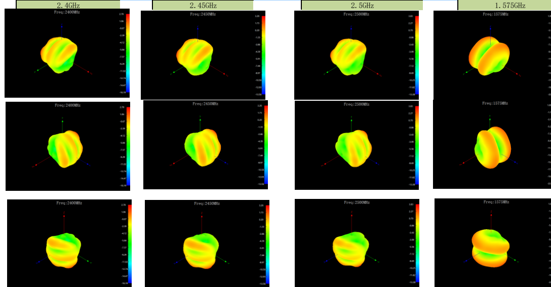
3D field pattern (xyz3 directions, marking the direction of the device under test)
