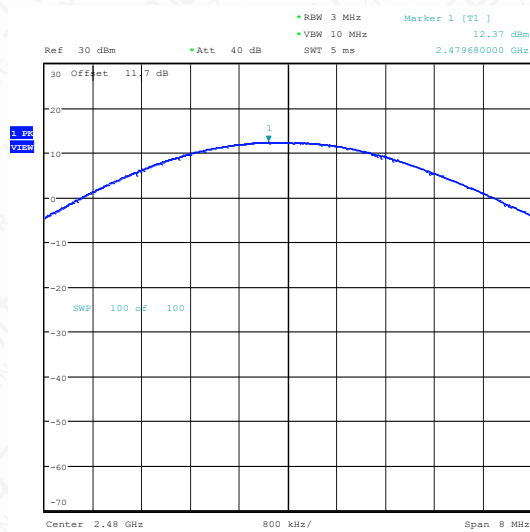
3DH5-Ant1-2480-PASS
