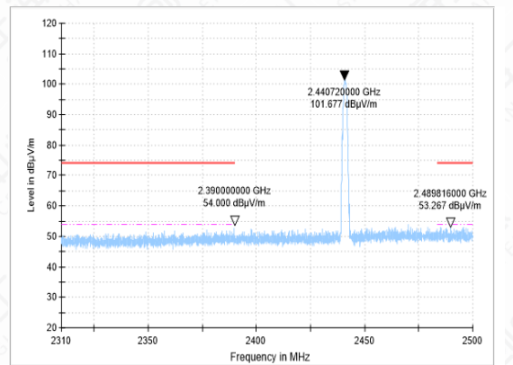
BANDEDGE-3DH5-CH39-PK
