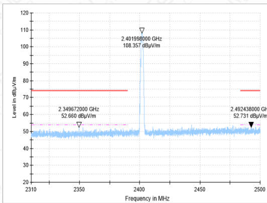
BANDEDGE-3DH5-CH0-PK
