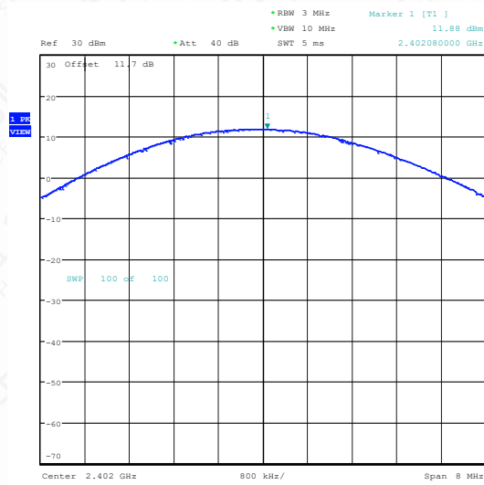
3DH5-Ant1-2402-PASS
