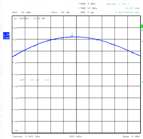
3DH5-Ant1-2441-PASS
