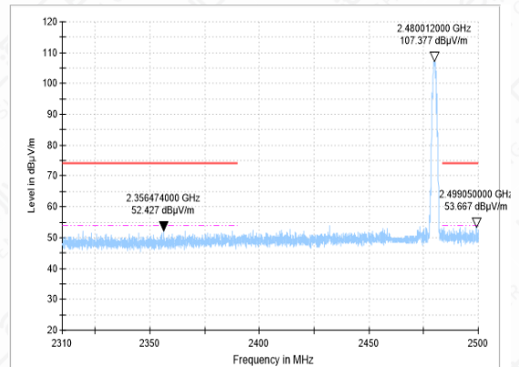
BANDEDGE-2DH5-CH78-PK
