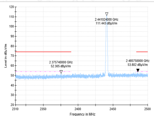
BANDEDGE-DH5-CH39-PK
