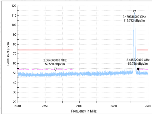
BANDEDGE-2DH5-CH39-PK
