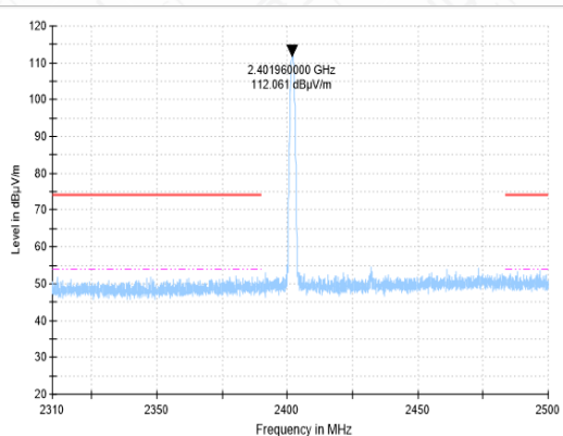
BANDEDGE-DH5-CH0-PK
