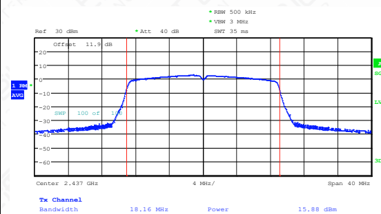
11N20SISO-Ant1-2437-PASS
