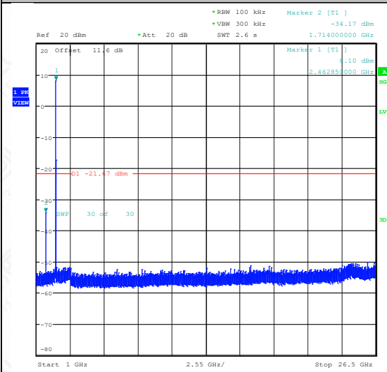
11B-Ant1-2462-1000~26500-PASS
