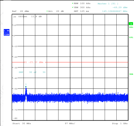
11N20SISO-Ant1-2462-30~1000-PASS
