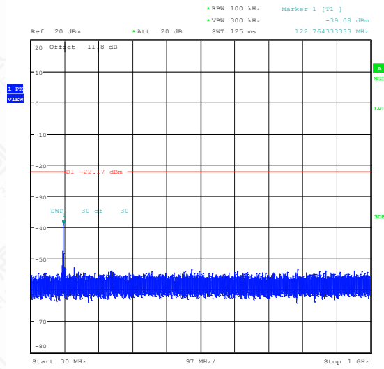
11B-Ant1-2437-30~1000-PASS
