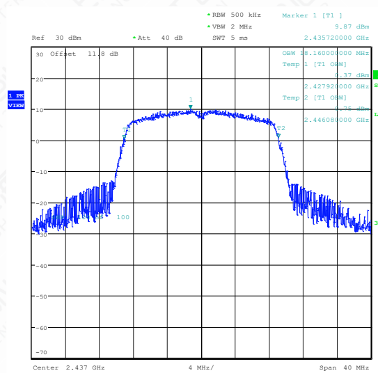
11N20SISO-Ant1-2437
