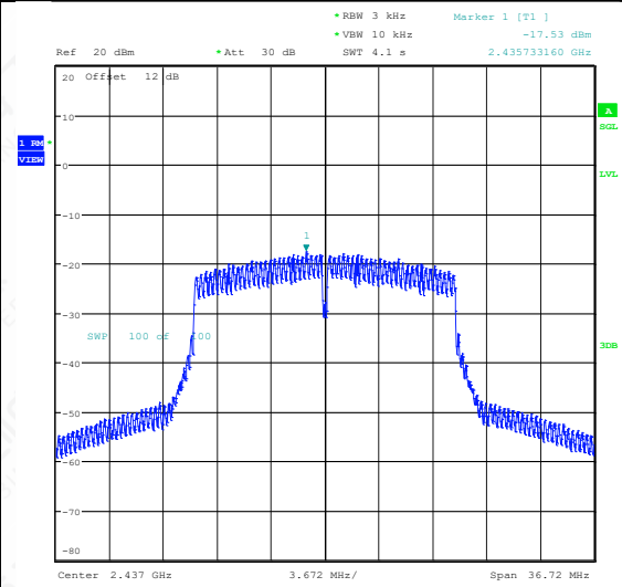
11N20SISO-Ant1-2437-PASS
