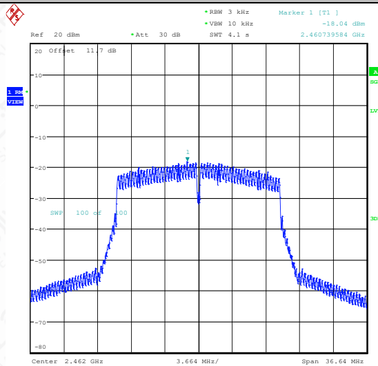
11N20SISO-Ant1-2462-PASS
