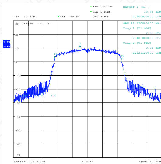
11N20SISO-Ant1-2412
