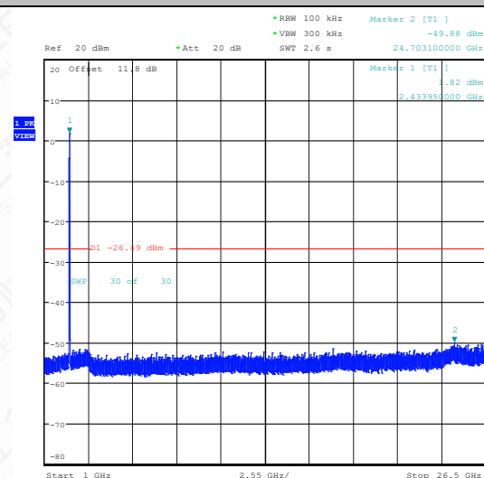
11G-Ant1-2437-1000~26500-PASS
