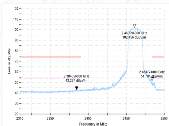
BANEDGE-11N-CH11-AV
