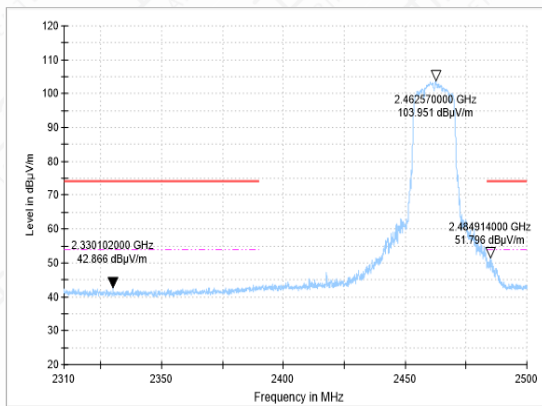
BANEDGE-11G-CH11-AV
