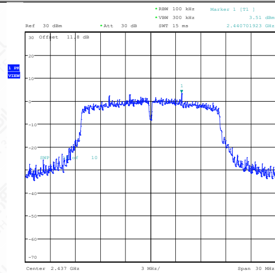
11G-Ant1-2437-0~Reference-PASS
