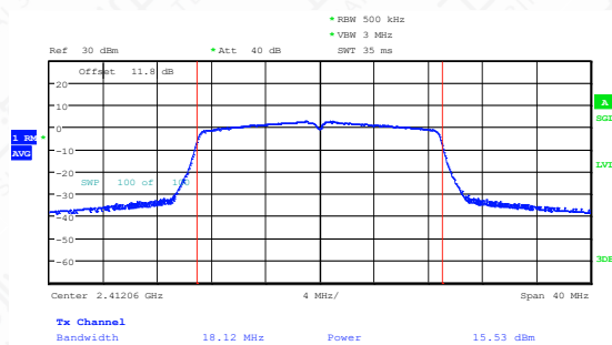
11N20SISO-Ant1-2412-PASS
