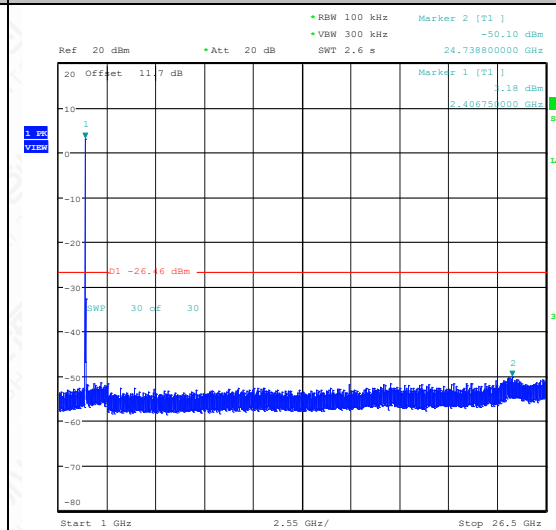
11G-Ant1-2412-1000~26500-PASS
