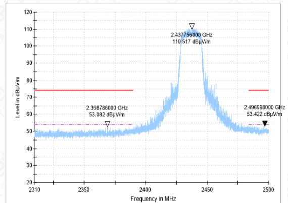
BANEDGE-11G-CH6-PK
