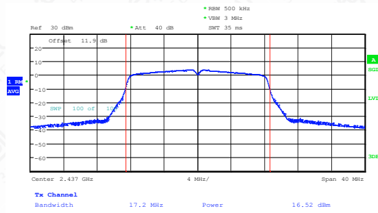
11G-Ant1-2437-PASS
