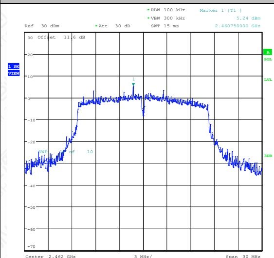
11G-Ant1-2462-0~Reference-PASS
