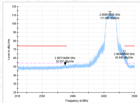
BANEDGE-11G-CH11-PK
