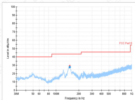
RSE-11G-CH11-30MHz-1GHz
