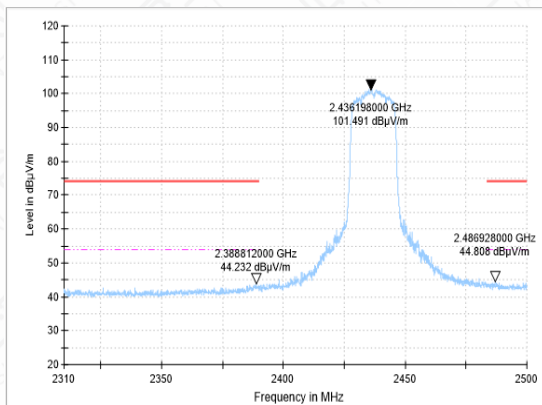
BANEDGE-11N-CH6-AV
