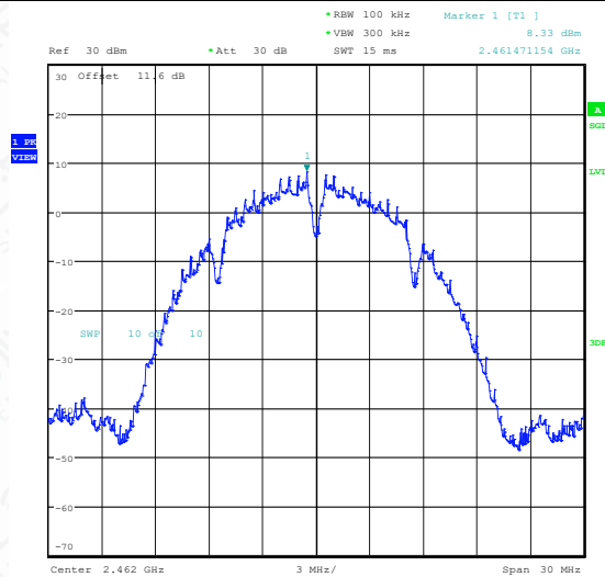
11B-Ant1-2462-0~Reference-PASS
