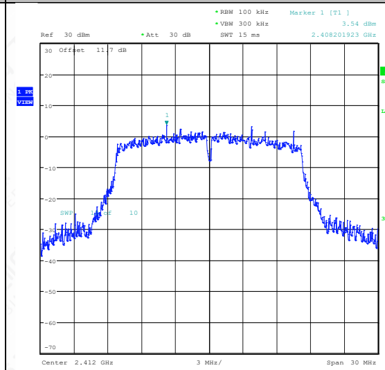
11G-Ant1-2412-0~Reference-PASS
