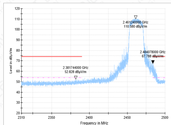
BANEDGE-11N-CH11-PK
