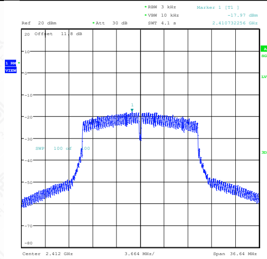
11N20SISO-Ant1-2412-PASS
