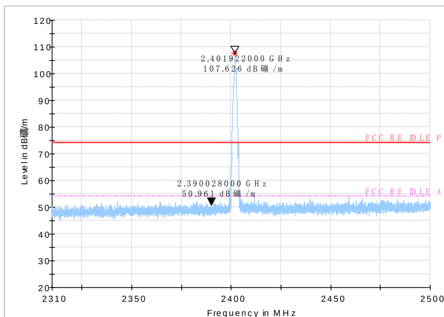
Fig.48 Bandedge (Low): \pi/4 DQPSK, low channel
