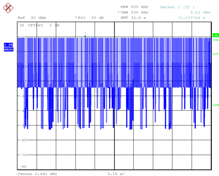
Fig.67 Time of occupancy (Dwell Time): Ch39,Packet 3-DH1
