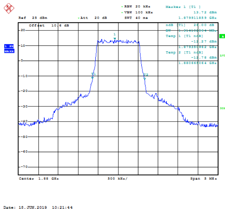
Fig.91 LTE band 2, 1.4MHz Bandwidth, QPSK (-26dBc BW)
