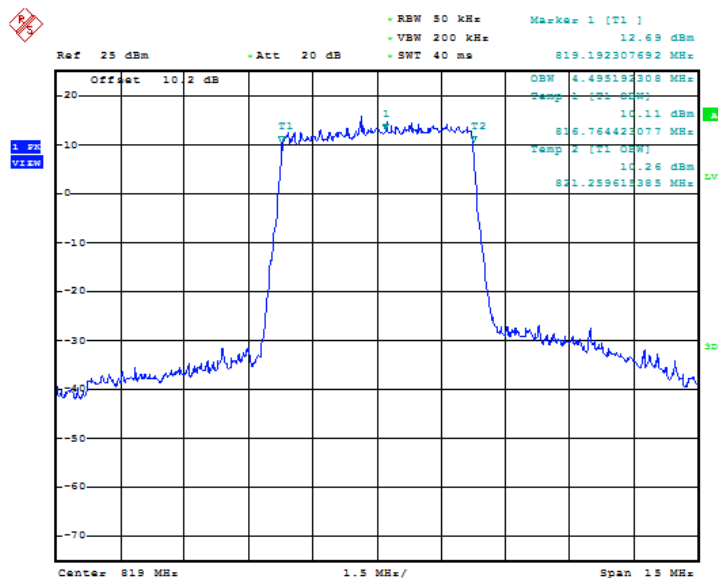
Fig.79 LTE band 26, 5MHz Bandwidth, QPSK (99% BW)
