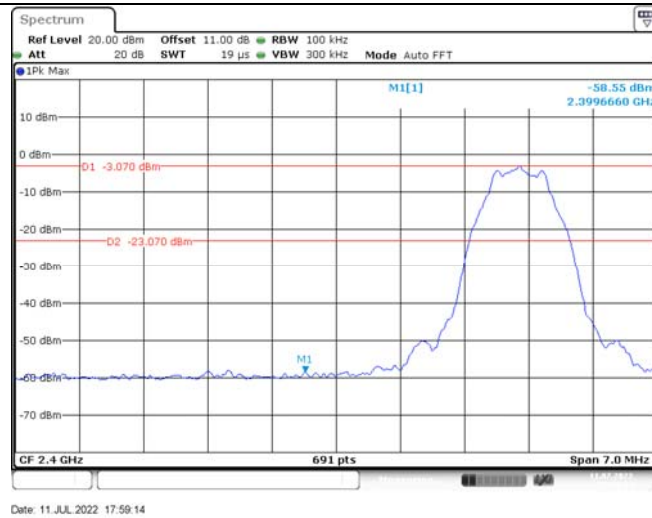
100 kHz Bandwidth of Frequency Band Edge
