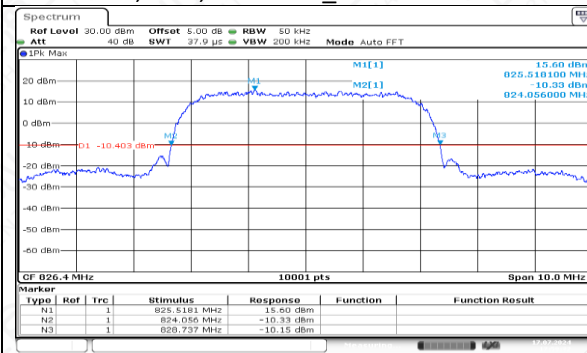
OB5,4132,826.4MHz_26dBDownOBW
