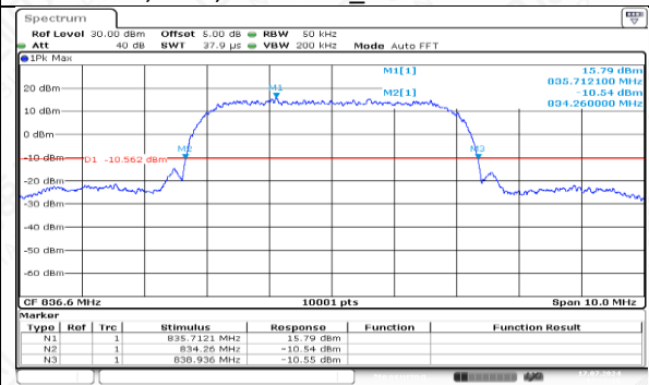
OB5,4183,836.6MHz_26dBDownOBW
