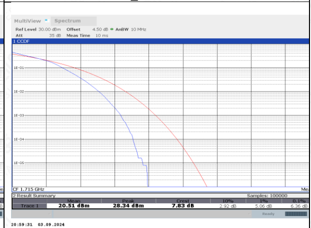
FDD04_LowRange_10MHz_1715_fullRB_16QAM
