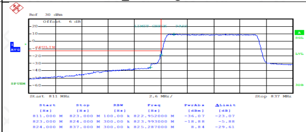
FDD05LowRange_10MHz_QPSK_FullRB_LowRange
