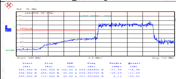
FDD12LowRange_10MHz_QPSK_FullRB_LowRange
