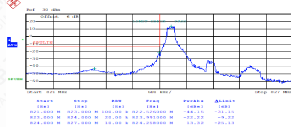
FDD05LowRange_1.4MHz_QPSK_1RB_LowRange
