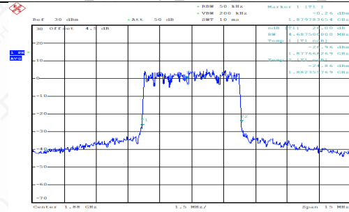
FDD02_MidRange_5MHz_1880MHz_16QAM
