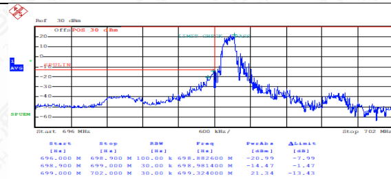
FDD12LowRange_1.4MHz_QPSK_1RB_LowRange
