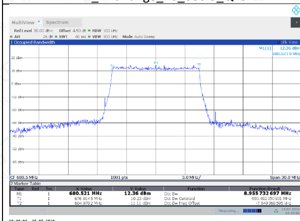
FDD71_MidRange_15_680.5_QPSK
