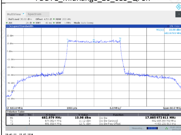
FDD71_MidRange_20_683_QPSK
