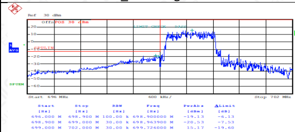
FDD12LowRange_1.4MHz_QPSK_FullRB_LowRange
