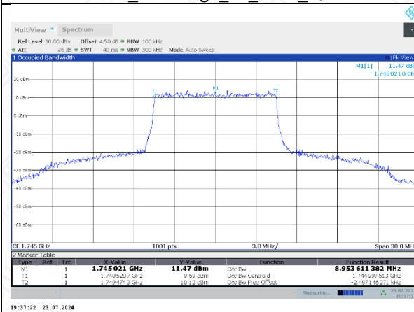
FDD66_MidRange_10_1745_QPSK
