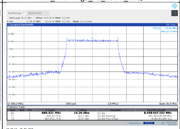
FDD71_MidRange_15_680.5_16QAM
