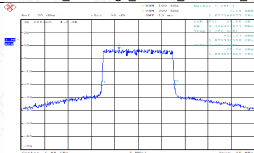
FDD02_MidRange_10MHz_1880MHz_QPSK
