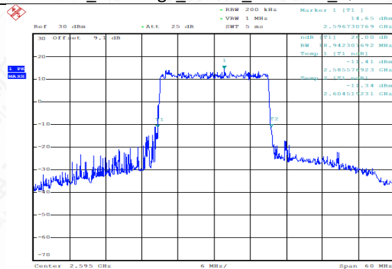
TDD38_MidRange_20MHz_2595MHz_QPSK
