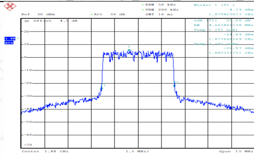
FDD02_MidRange_5MHz_1880MHz_QPSK
