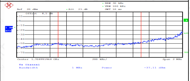
FDD04_LowRange_1.4_1708995968Hz_1RB_LowRangeOut of Limit Channel Power
