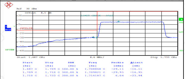
FDD04LowRange_20MHz_QPSK_FullRB_LowRange
