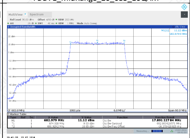
FDD71_MidRange_20_683_16QAM
