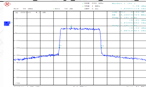
FDD02_MidRange_15MHz_1880MHz_16QAM
