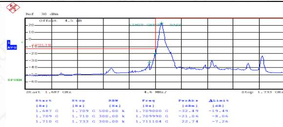
FDD04LowRange_20MHz_QPSK_1RB_LowRange
