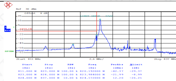
FDD05LowRange_10MHz_QPSK_1RB_LowRange
