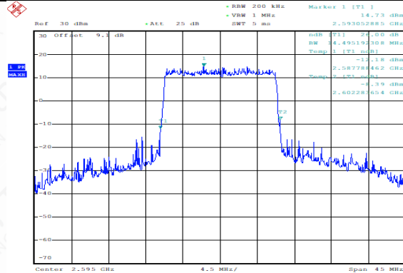
TDD38_MidRange_15MHz_2595MHz_QPSK
