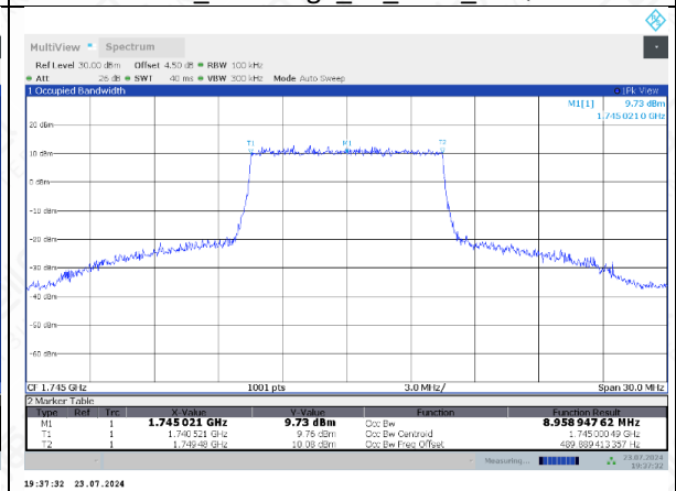
FDD66_MidRange_10_1745_16QAM
