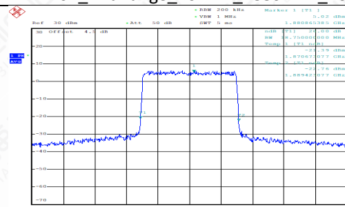
FDD02_MidRange_20MHz_1880MHz_16QAM
