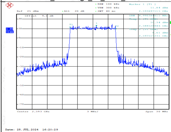
TDD41_MidRange_10_2593_16QAM
