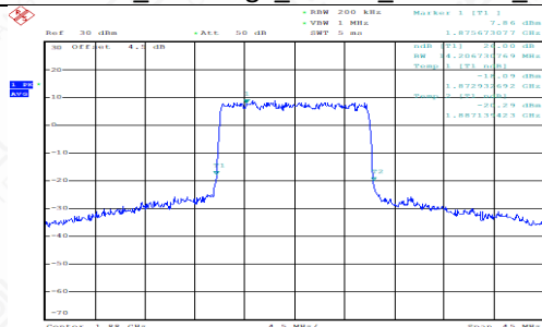
FDD02_MidRange_15MHz_1880MHz_QPSK
