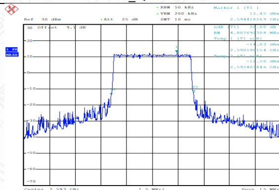
TDD41_MidRange_5MHz_2593MHz_QPSK
