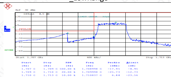
FDD04LowRange_1.4MHz_QPSK_FullRB_LowRange
