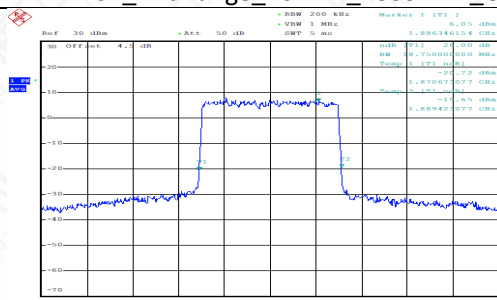
FDD02_MidRange_20MHz_1880MHz_QPSK
