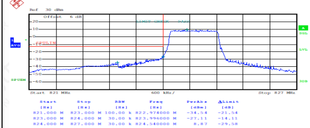
FDD05LowRange_1.4MHz_QPSK_FullRB_LowRange
