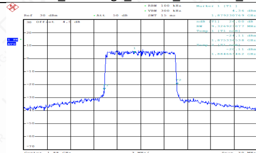
FDD02_MidRange_10MHz_1880MHz_16QAM
