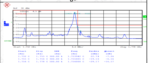
FDD04HighRange_20MHz_QPSK_1RB_HighRange
