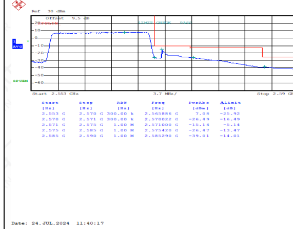
FDD07HighRange_20MHz_QPSK_FullRB_HighRange
