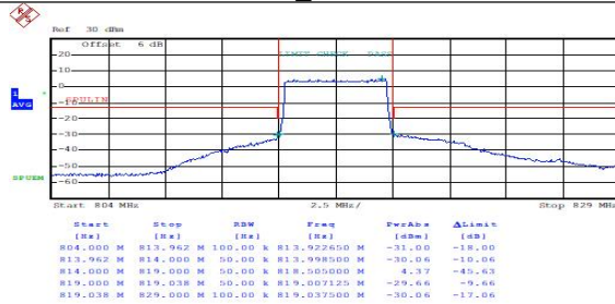
FDD26(Part 90)Low_5MHz_QPSK_FullRB Low
