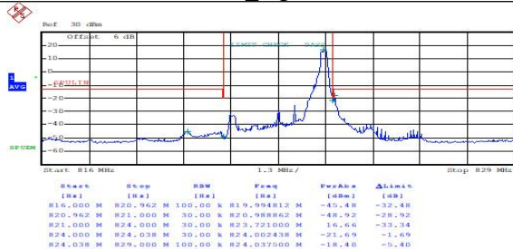
FDD26(Part 90)_High_3MHz_QPSK_1RB high
