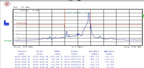
FDD26(Part 90)_High_5MHz_QPSK_1RB high
