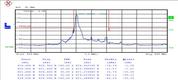
FDD26(Part 90)_High_3MHz_QPSK_1RB low
