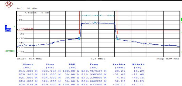
FDD26(Part 90)_High_3MHz_QPSK_FullRB High
