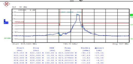
FDD26(Part 90)_High_1.4MHz_QPSK_1RB high
