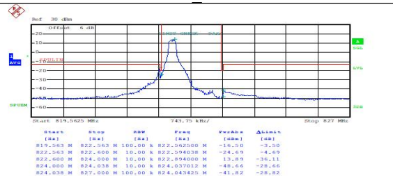
FDD26(Part 90)_High_1.4MHz_QPSK_1RB low
