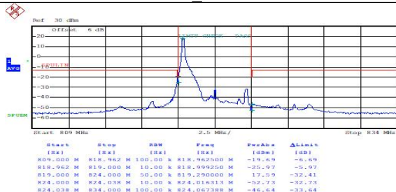
FDD26(Part 90)_High_5MHz_QPSK_1RB low
