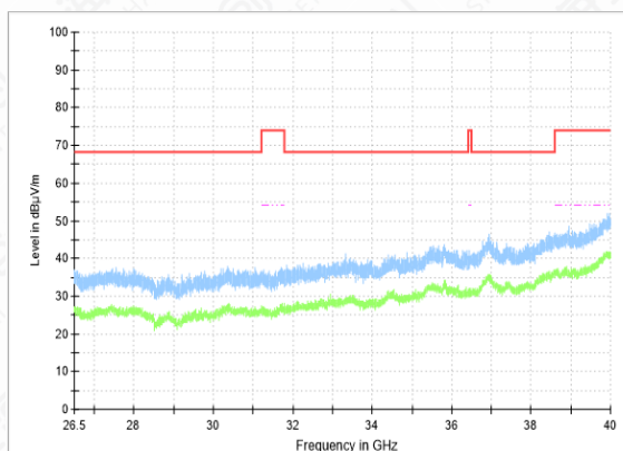
RSE-11N(40M)-CH38-26.5GHz-40GHz
