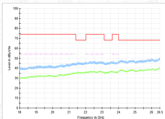
RSE-11N(20M)-CH120-18GHz-26.5GHz
