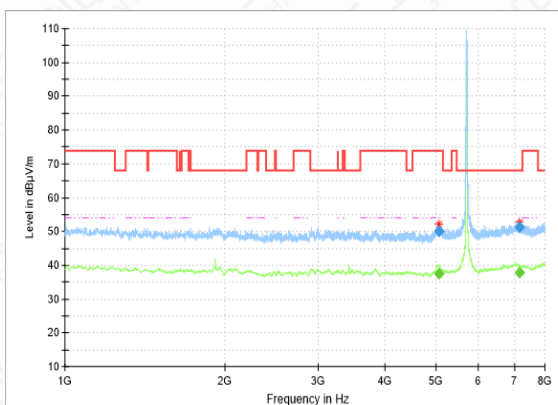
RSE-11A-CH140-1GHz-8GHz
