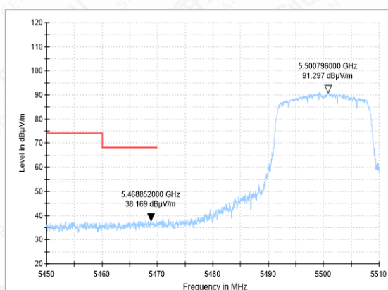
Bandedge-11A-CH100-AV
