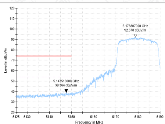
Bandedge-11N(20M)-CH36-AV
