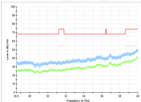
RSE-11A-CH52-26.5GHz-40GHz
