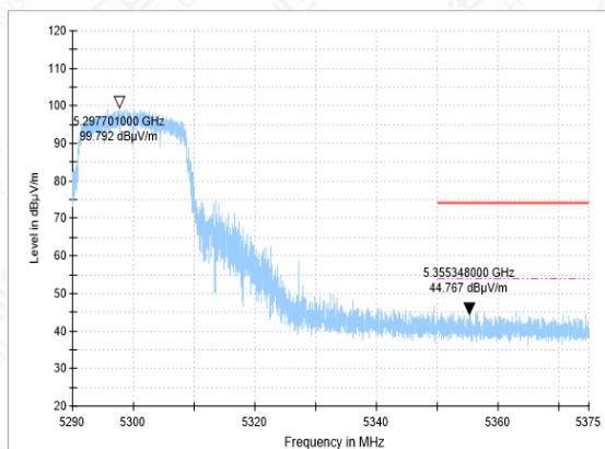
Bandedge-11N(20M)-CH60-PK
