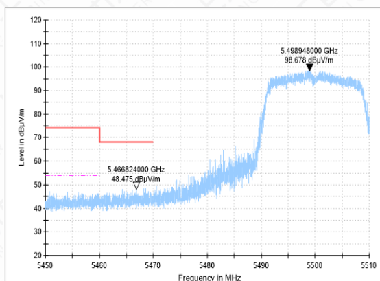
Bandedge-11AC(20M)-CH100-PK
