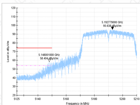
Bandedge-11AC(40M)-CH38-PK
