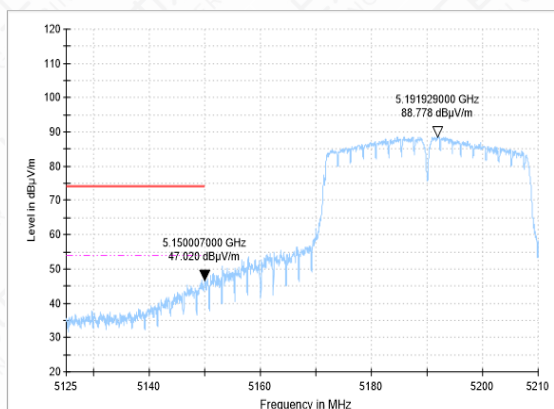
Bandedge-11N(40M)-CH38-AV
