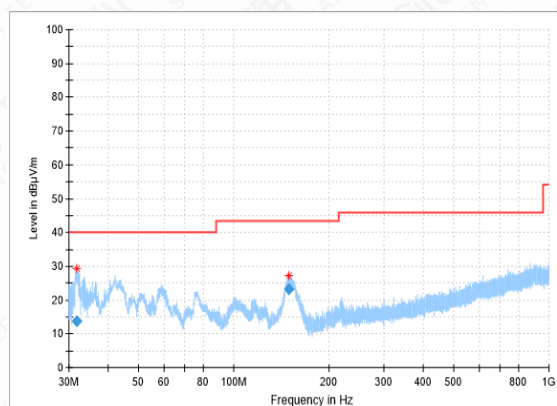
RSE-11N(20M)-CH36-30MHz-1GHz
