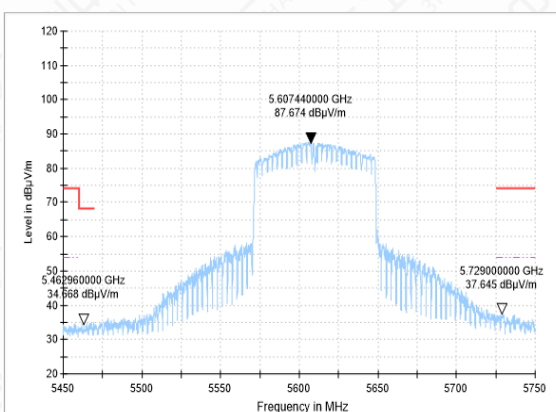
Bandedge-11AC(80M)-CH122-AV
