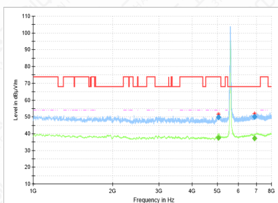
RSE-11N(40M)-CH118-1GHz-8GHz
