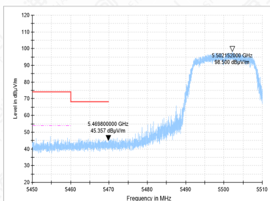
Bandedge-11A-CH100-PK
