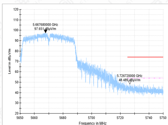
Bandedge-11AC(40M)-CH134-PK
