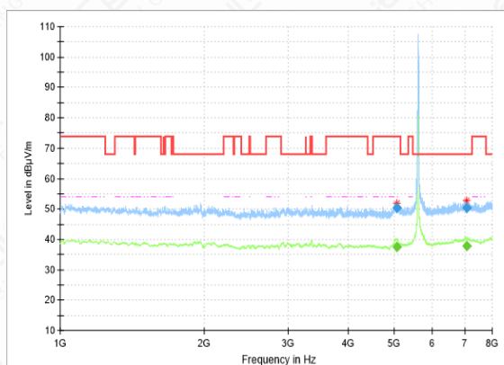
RSE-11N(20M)-CH120-1GHz-8GHz
