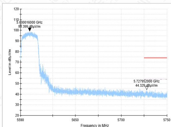
Bandedge-11AC(20M)-CH120-PK
