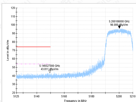
Bandedge-11AC(20M)-CH40-PK
