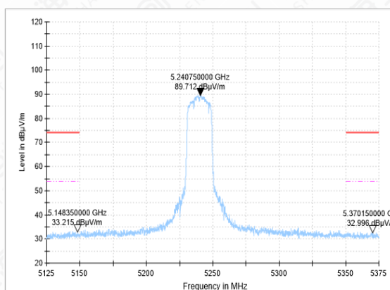
Bandedge-11AC(20M)-CH48-AV
