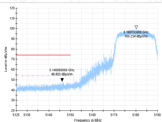
Bandedge-11N(20M)-CH36-PK
