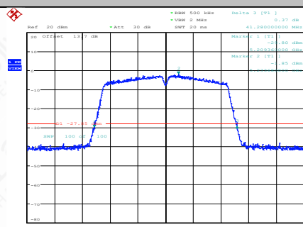
11AC40SISO-Ant1-5230
