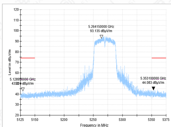
Bandedge-11N(40M)-CH54-PK
