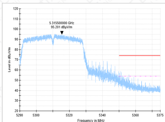
Bandedge-11N(40M)-CH62-PK
