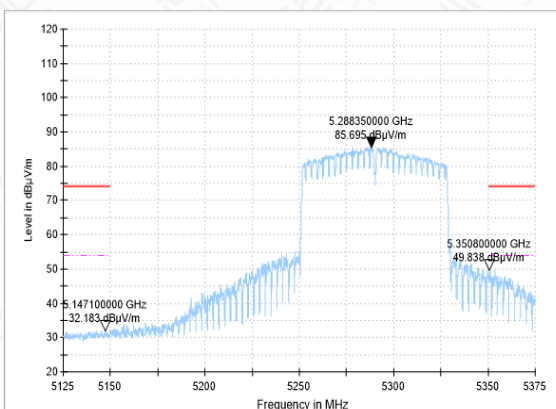
Bandedge-11AC(80M)-CH58-AV
