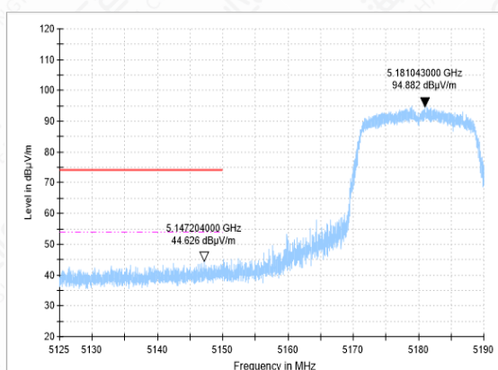
Bandedge-11AC(20M)-CH36-PK
