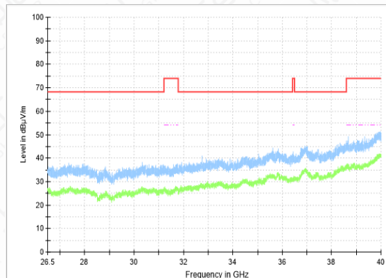
RSE-11N(20M)-CH36-26.5GHz-40GHz
