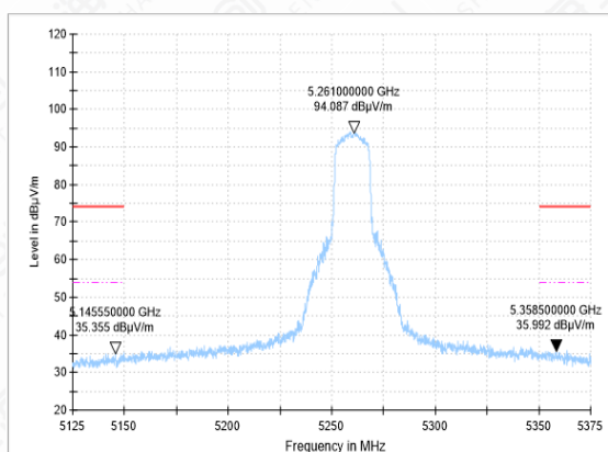
Bandedge-11A-CH52-AV
