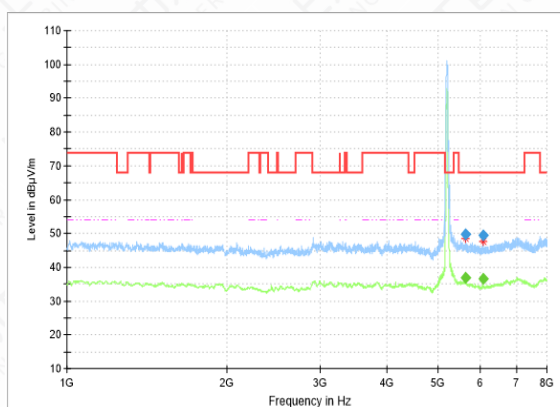
RSE-11N(40M)-CH62-1GHz-8GHz
