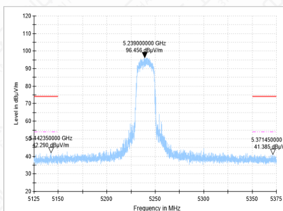
Bandedge-11AC(20M)-CH48-PK
