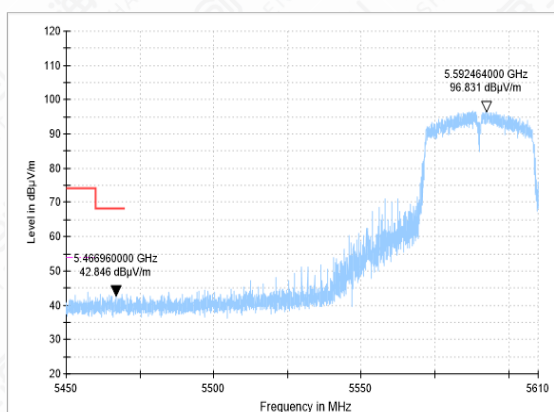
Bandedge-11N(40M)-CH118-PK
