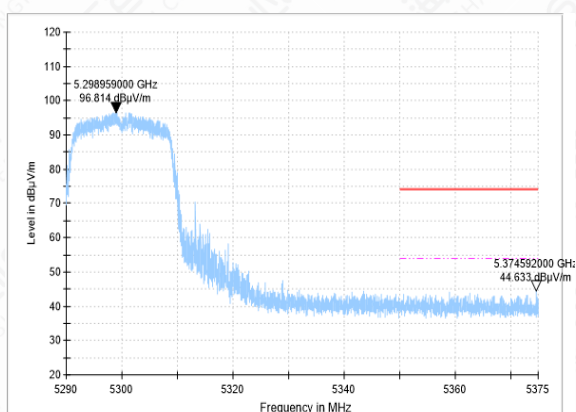
Bandedge-11AC(20M)-CH60-PK
