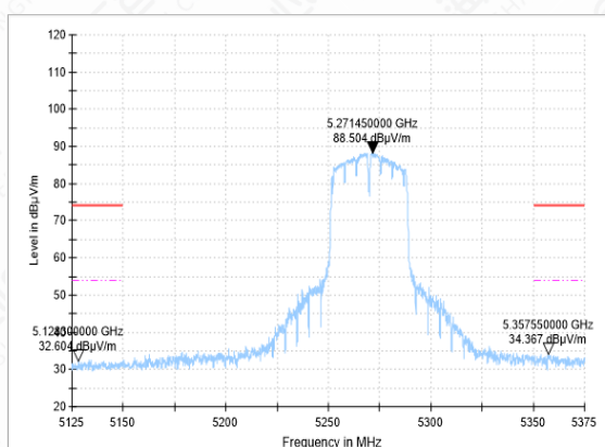
Bandedge-11AC(40M)-CH54-AV
