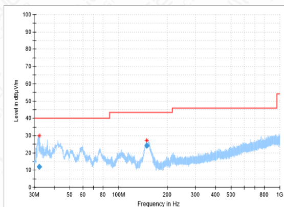
RSE-11N(20M)-CH120-30MHz-1GHz
