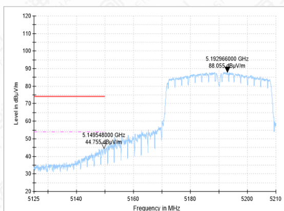
Bandedge-11AC(40M)-CH38-AV
