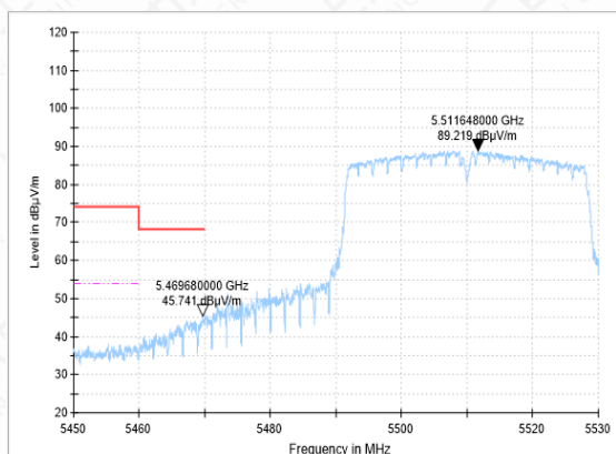
Bandedge-11AC(40M)-CH102-AV
