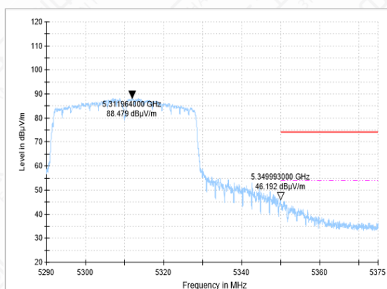
Bandedge-11N(40M)-CH62-AV
