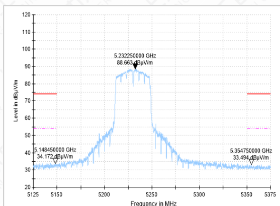
Bandedge-11AC(40M)-CH46-AV
