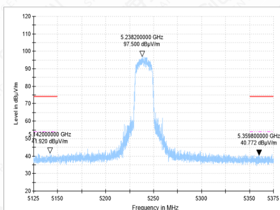
Bandedge-11N(20M)-CH48-PK
