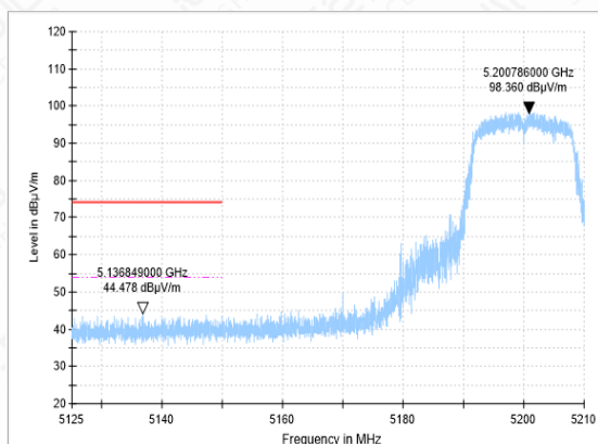
Bandedge-11A-CH40-PK
