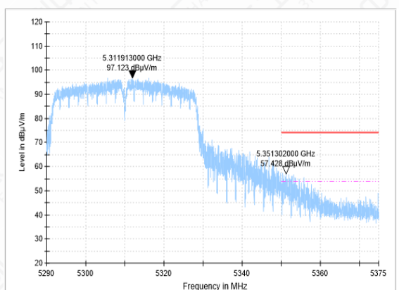
Bandedge-11AC(40M)-CH62-PK
