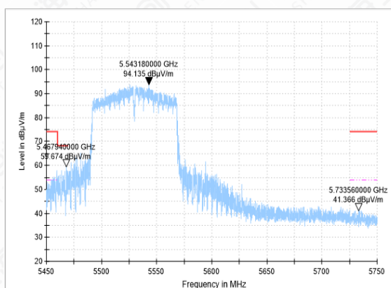
Bandedge-11AC(80M)-CH106-PK
