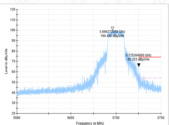
Bandedge-11N(20M)-CH140-PK
