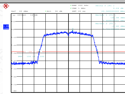
11AC20SISO-Ant1-5700
