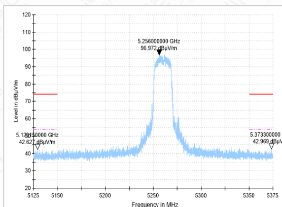
Bandedge-11AC(20M)-CH52-PK
