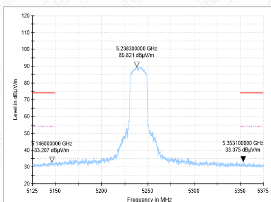
Bandedge-11N(20M)-CH48-AV
