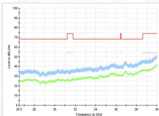
RSE-11N(20M)-CH120-26.5GHz-40GHz
