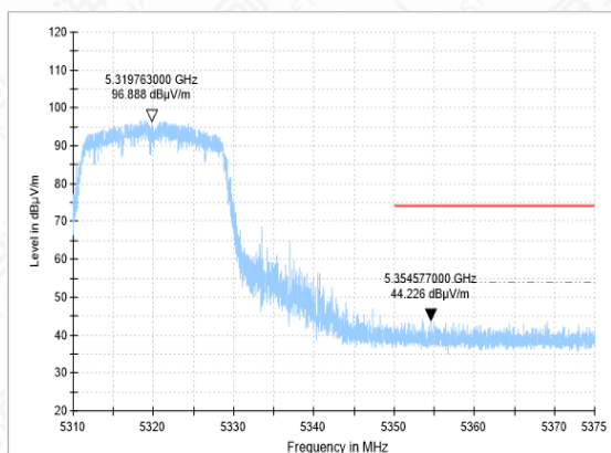
Bandedge-11N(20M)-CH64-PK
