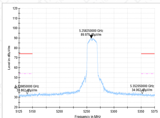
Bandedge-11AC(20M)-CH52-AV
