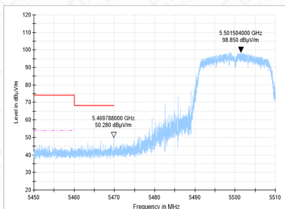
Bandedge-11N(20M)-CH100-PK
