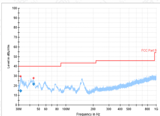
RSE-11A-CH140-30MHz-1GHz
