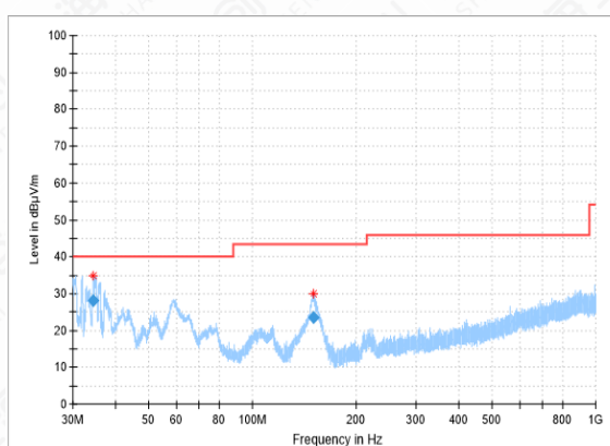
RSE-11N(40M)-CH118-30MHz-1GHz
