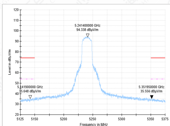
Bandedge-11A-CH48-AV
