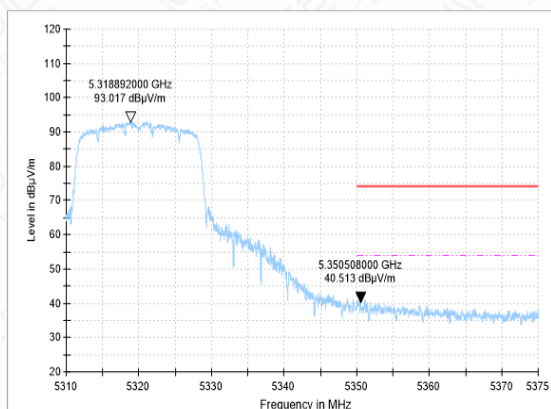
Bandedge-11A-CH64-AV
