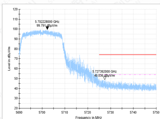
Bandedge-11AC(20M)-CH140-PK
