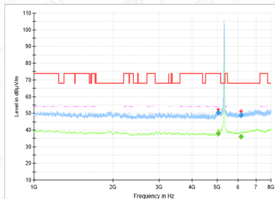
RSE-11N(20M)-CH60-1GHz-8GHz
