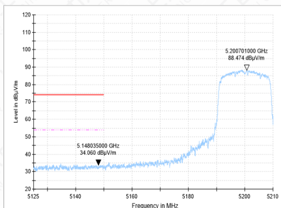
Bandedge-11N(20M)-CH40-AV
