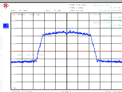
11AC20SISO-Ant1-5500
