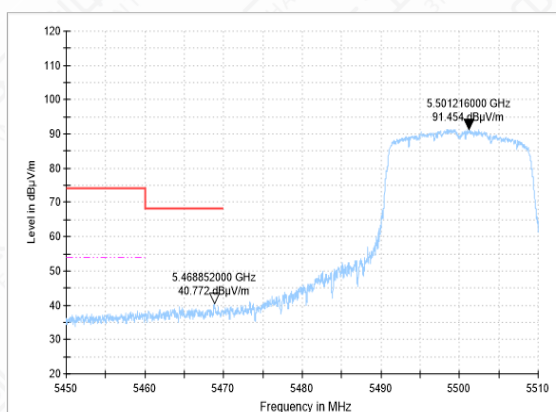
Bandedge-11AC(20M)-CH100-AV
