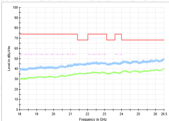
RSE-11N(20M)-CH36-18GHz-26.5GHz
