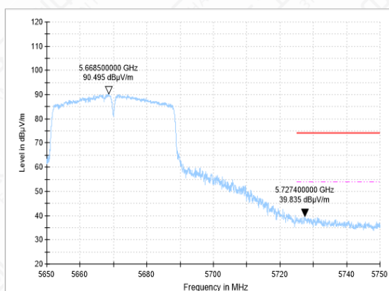
Bandedge-11N(40M)-CH134-AV
