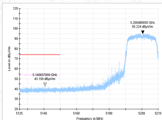
Bandedge-11N(20M)-CH40-PK
