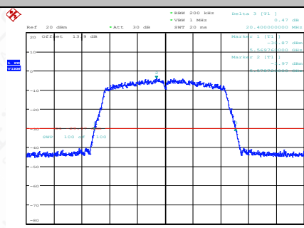
11AC20SISO-Ant1-5580
