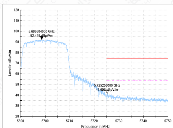
Bandedge-11AC(20M)-CH140-AV
