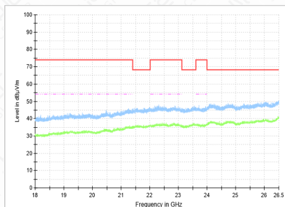
RSE-11A-CH140-18GHz-26.5GHz
