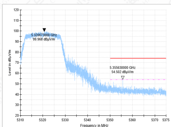
Bandedge-11A-CH64-PK
