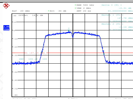
11AC40SISO-Ant1-5310
