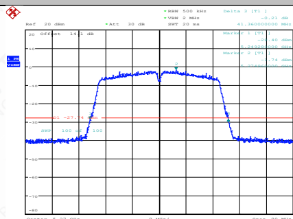
11AC40SISO-Ant1-5270
