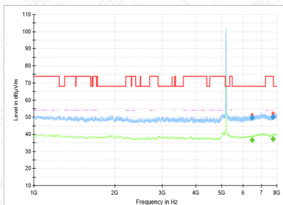
RSE-11N(20M)-CH36-1GHz-8GHz
