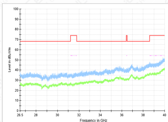
RSE-11A-CH140-26.5GHz-40GHz
