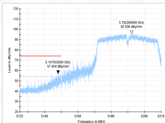
Bandedge-11N(40M)-CH38-PK
