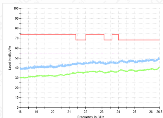
RSE-11N(20M)-CH60-18GHz-26.5GHz
