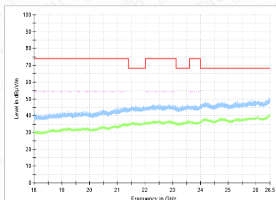
RSE-11N(40M)-CH38-18GHz-26.5GHz
