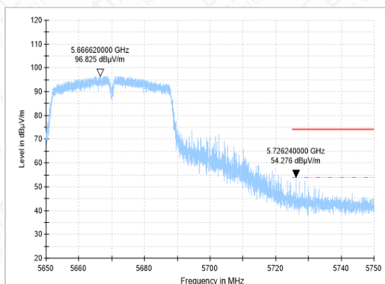
Bandedge-11N(40M)-CH134-PK
