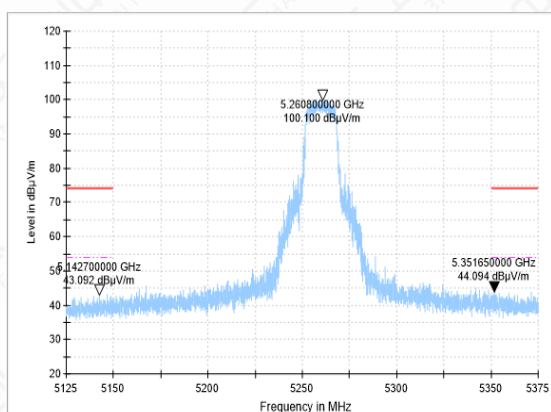
Bandedge-11A-CH52-PK
