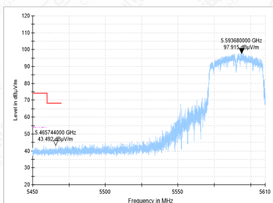
Bandedge-11AC(40M)-CH118-PK
