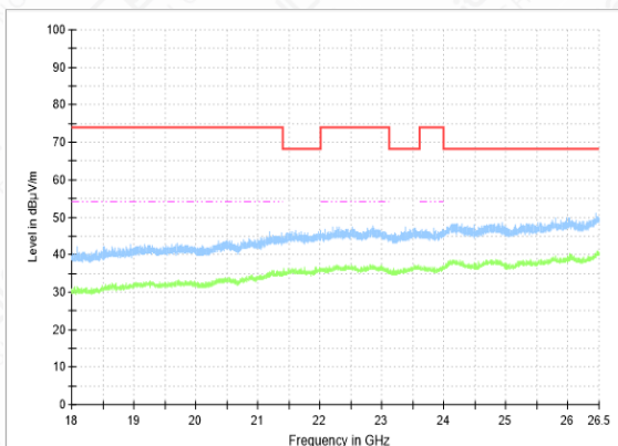
RSE-11A-CH52-18GHz-26.5GHz
