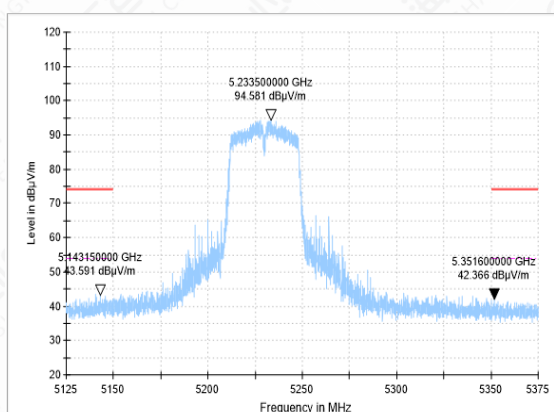
Bandedge-11N(40M)-CH46-PK
