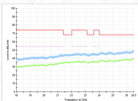
RSE-11N(40M)-CH62-18GHz-26.5GHz
