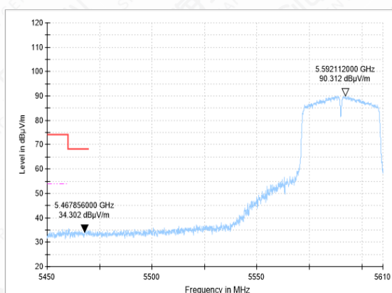
Bandedge-11N(40M)-CH118-AV
