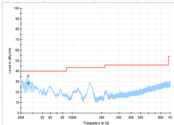
RSE-11N(40M)-CH38-30MHz-1GHz
