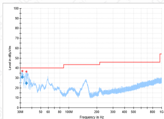
RSE-11N(40M)-CH62-30MHz-1GHz
