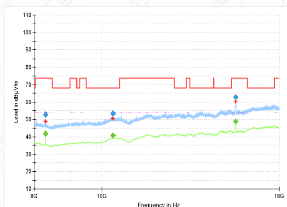
RSE-11N(40M)-CH38-8GHz-18GHz
