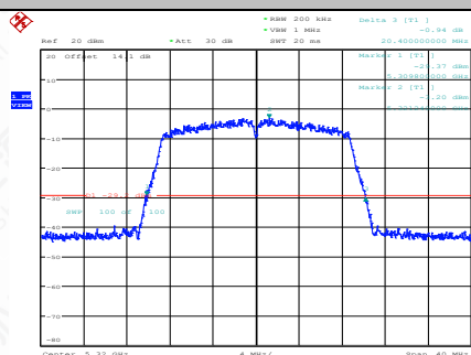
11AC20SISO-Ant1-5320
