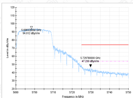
Bandedge-11N(20M)-CH140-AV
