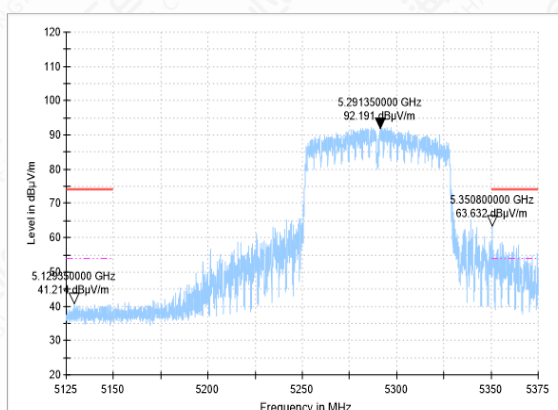
Bandedge-11AC(80M)-CH58-PK
