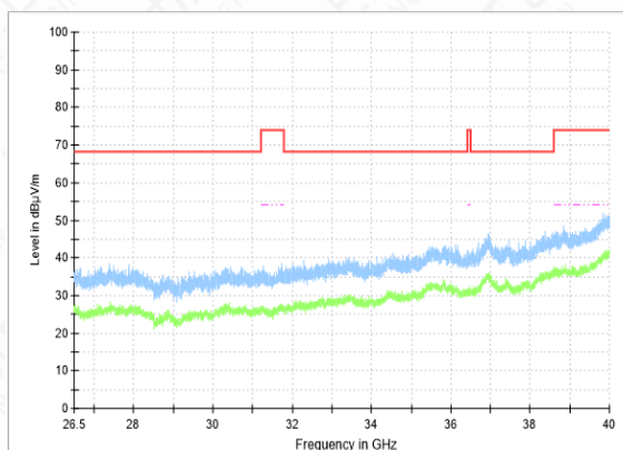
RSE-11N(20M)-CH60-26.5GHz-40GHz
