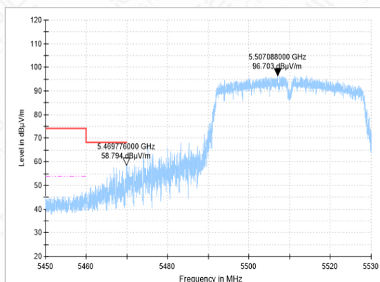
Bandedge-11AC(40M)-CH102-PK
