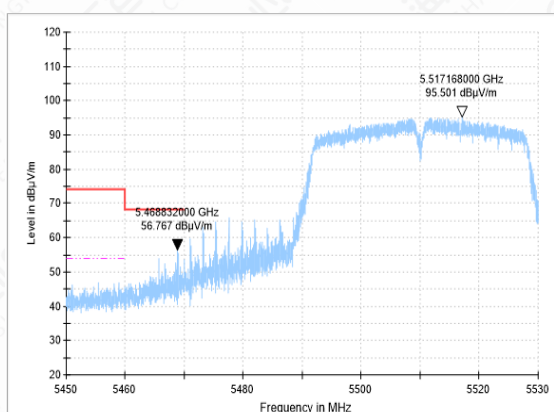
Bandedge-11N(40M)-CH102-PK
