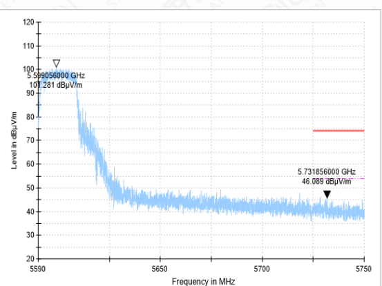
Bandedge-11N(20M)-CH120-PK
