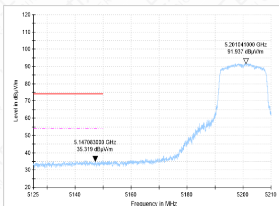
Bandedge-11A-CH40-AV
