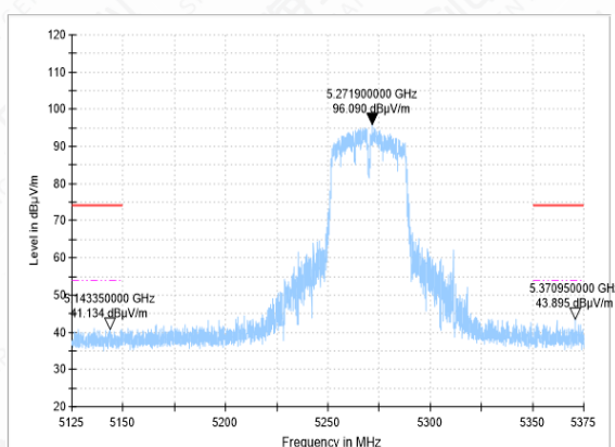
Bandedge-11AC(40M)-CH54-PK
