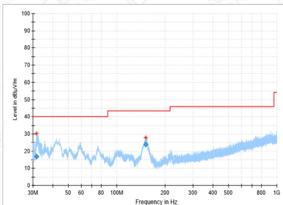
RSE-11N(20M)-CH60-30MHz-1GHz
