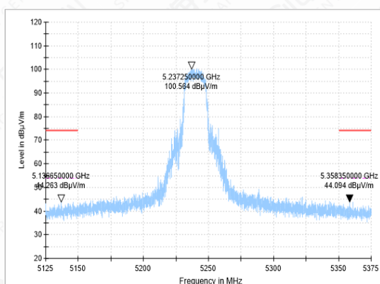
Bandedge-11A-CH48-PK
