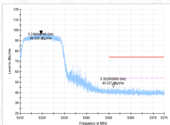
Bandedge-11AC(20M)-CH64-PK
