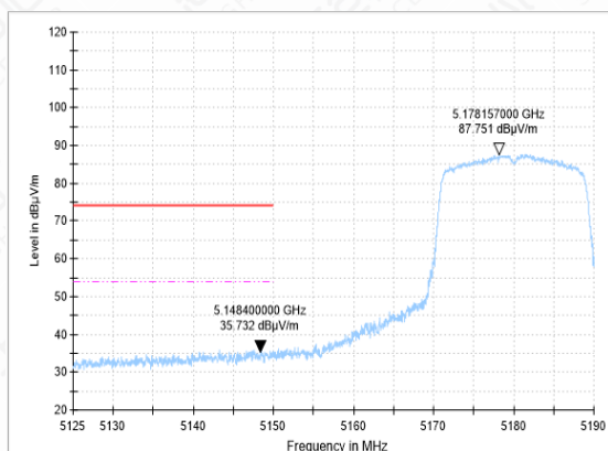
Bandedge-11AC(20M)-CH36-AV
