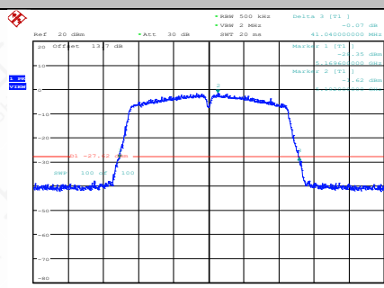
11AC40SISO-Ant1-5190
