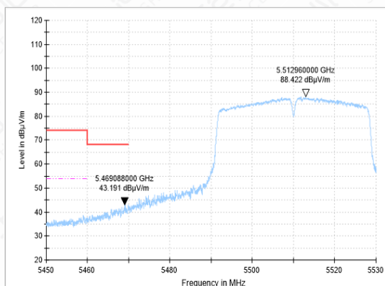
Bandedge-11N(40M)-CH102-AV
