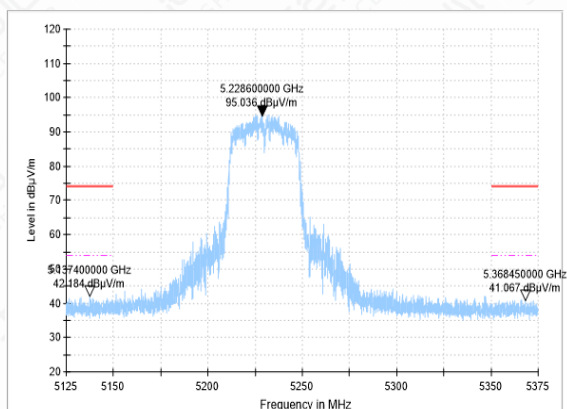
Bandedge-11AC(40M)-CH46-PK
