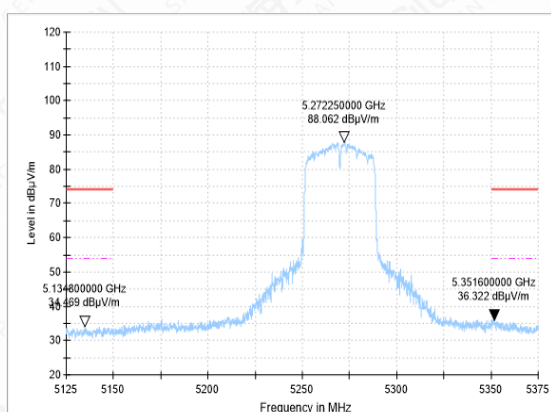
Bandedge-11N(40M)-CH54-AV
