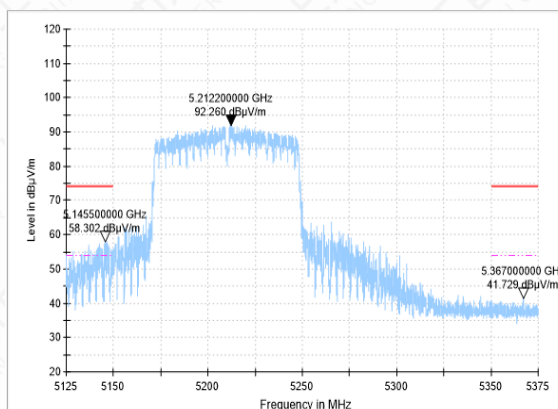
Bandedge-11AC(80M)-CH42-PK
