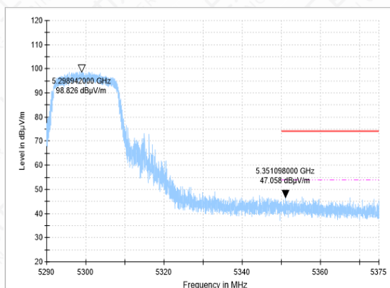
Bandedge-11A-CH60-PK
