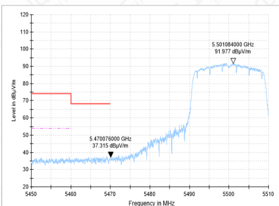
Bandedge-11N(20M)-CH100-AV
