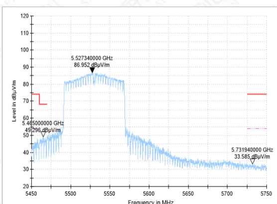
Bandedge-11AC(80M)-CH106-AV
