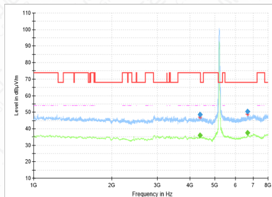
RSE-11N(40M)-CH38-1GHz-8GHz
