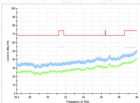
RSE-11N(40M)-CH62-26.5GHz-40GHz
