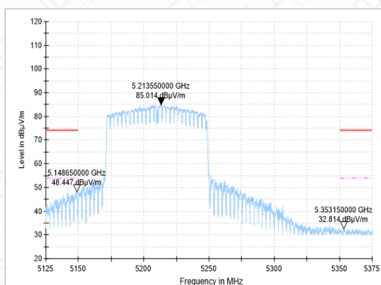
Bandedge-11AC(80M)-CH42-AV
