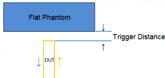
Figure 15.4-1 Proximity sensor triggering distances assessment(Right side)
